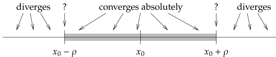
Figure 2.10: Convergence of a power series.
