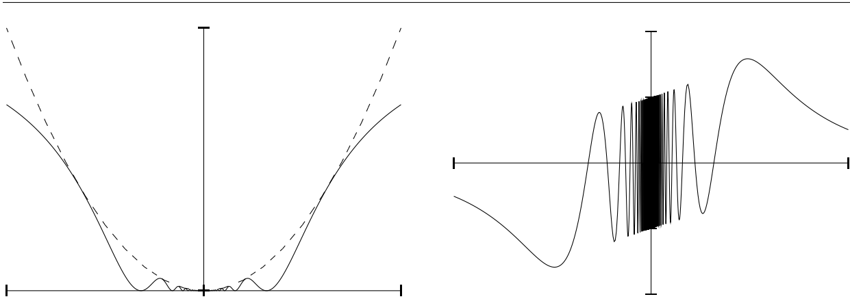
Figure 4.7: A function with a discontinuous derivative. The function f is on the left and f' is on the right. Notice that f(x) \leq x^2 on the left graph.
