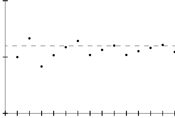
Figure 2.9: The first 14 partial sums of the rearrangement converging to 1.2.
