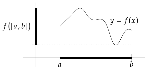
Figure 3.8: The image of a continuous f: [a, b] \rightarrow \mathbb{R} .
