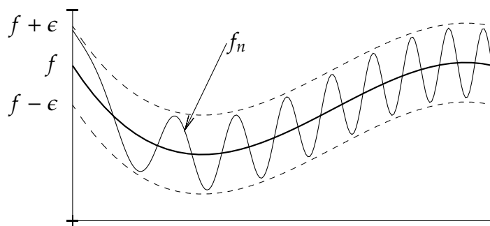
Figure 6.3: In uniform convergence, for n \geq N , the functions f_n are within a strip of \pm\epsilon from f .
