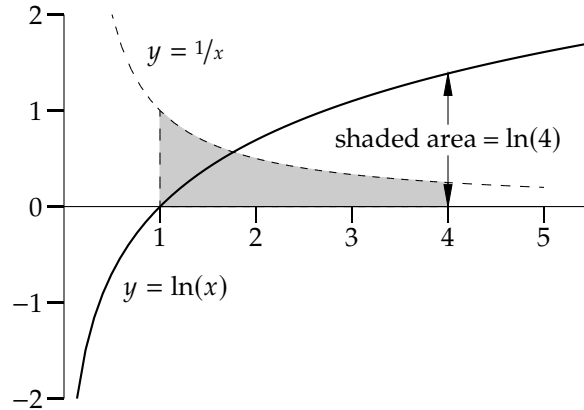
Figure 5.6: Plot of \ln(x) together with 1/x , showing the value \ln(4) .
