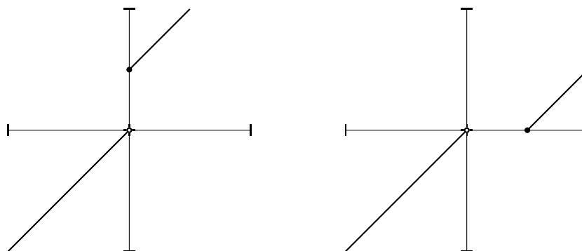
Figure 3.13: Graph of f on the left and f^{-1} on the right.
