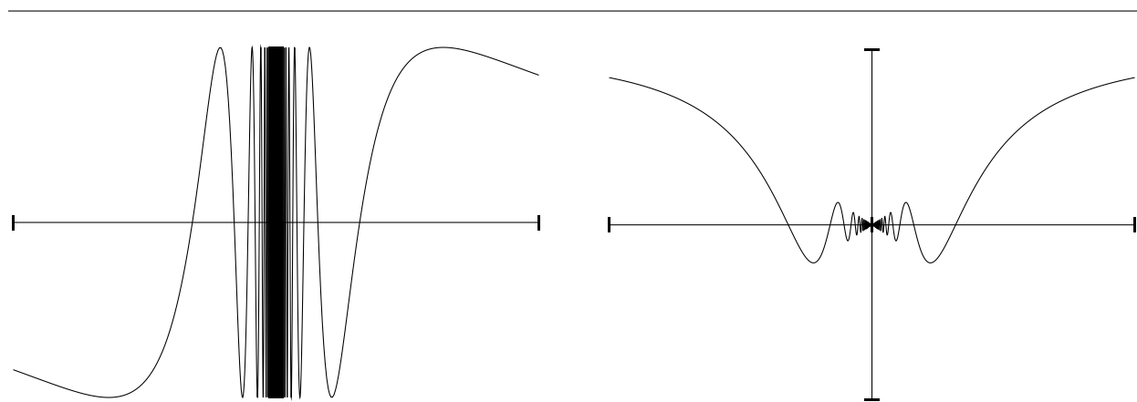
Figure 3.2: Graphs of \sin(1/x) and x \sin(1/x) . Note that the computer cannot properly graph \sin(1/x) near zero as it oscillates too fast.
