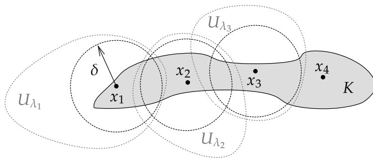
Figure 7.13: Covering K by U_\lambda . The points x_1, x_2, x_3, x_4 , the three sets U_{\lambda_1}, U_{\lambda_2}, U_{\lambda_3} , and the first three balls of radius \delta are drawn.
