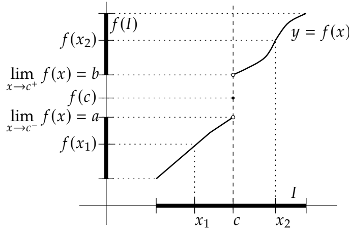
Figure 3.11: Increasing function f: I \rightarrow \mathbb{R} discontinuity at c .
