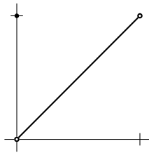
Figure 3.1: Function with a different limit and value at 0.
