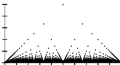
Figure 3.5: Graph of the “popcorn function.”
