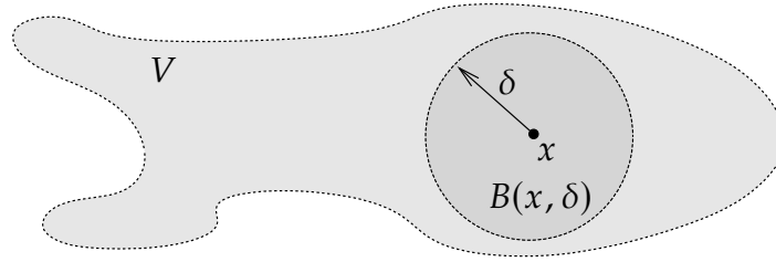
Figure 7.5: Open set in a metric space. Note that \delta depends on x .
