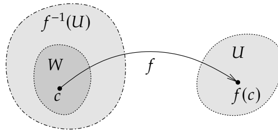
Figure 7.15: For every neighborhood U of f(c) , the set f^{-1}(U) contains an open neighborhood W of c .
