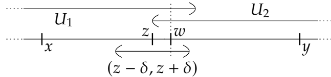
Figure 7.8: Proof that an interval is connected.
