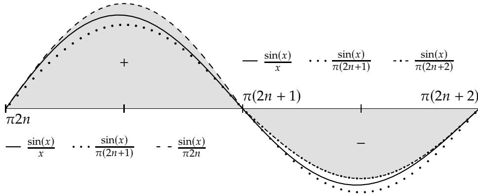
Figure 5.9: Bound of \int_{2\pi n}^{2\pi(n+1)} \frac{\sin(x)}{x} dx using the shaded integral (signed area \frac{1}{\pi n} + \frac{-1}{\pi(n+1)} ).
