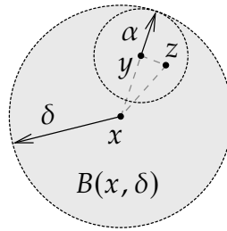
Figure 7.6: Proof that B(x, \delta) is open: B(y, \alpha) \subset B(x, \delta) with the triangle inequality illustrated.
