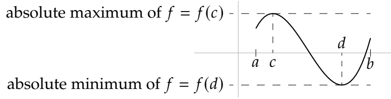
Figure 3.6: f: [a, b] \rightarrow \mathbb{R} achieves an absolute maximum f(c) at c , and an absolute minimum f(d) at d .
