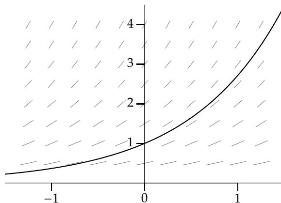
Figure 5.7: Plot of e^x , together with a slope field giving slope y at every point (x, y) . The equation \frac{d}{dx}e^x = e^x means that y = e^x follows these slopes.
