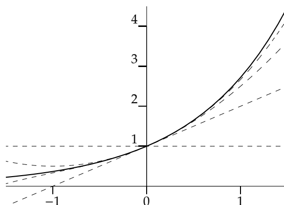
Figure 6.9: The exponential (solid line) together with f_0, f_1, f_2, f_3 (dashed).
