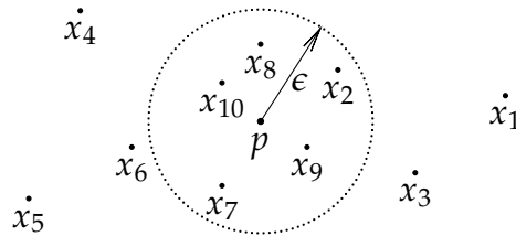
Figure 7.10: Sequence converging to p . The first 10 points are shown and M = 7 for this \epsilon .
