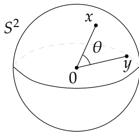
Figure 7.4: The great circle distance on the unit sphere.
