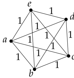
Figure 7.3: Sample discrete metric space \{a, b, c, d, e\} , the distance between any two points is 1.
