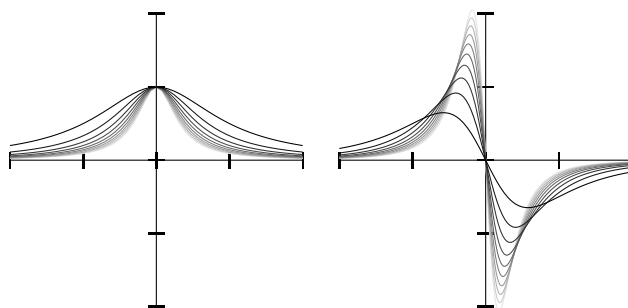
Figure 6.7: Graphs of \frac{1}{1+nx^2} and its derivative for n = 1, 2, \dots, 10 , with higher n in lighter gray.
