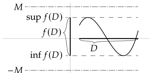
Figure 1.4: Example of a bounded function, a bound M , and its supremum and infimum.
