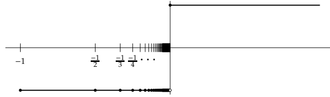
Figure 3.4: Jump discontinuity. The values of f(-1/n) and f(0) are marked as black dots.
