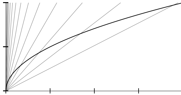
Figure 3.10: Graph of \sqrt{x} and some secant lines through (0, 0) and (x, \sqrt{x}) .
