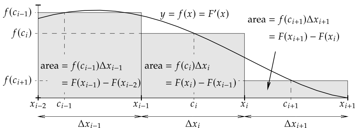
Figure 5.5: Mean value theorem on subintervals of a partition approximating the area under the curve.
