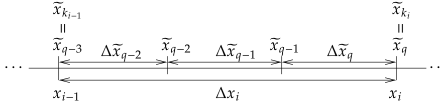
Figure 5.2: Refinement of a subinterval. Notice \Delta x_i = \Delta \tilde{x}_{q-2} + \Delta \tilde{x}_{q-1} + \Delta \tilde{x}_q , and also k_{i-1} + 1 = q - 2 and k_i = q .
