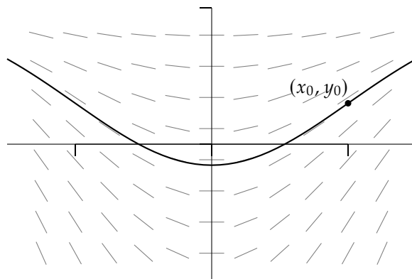
Figure 6.8: A slope field giving the slope F(x, y) at each point, in this case F(x, y) = x(1 - y) . A solution is drawn going through the point (x_0, y_0) = (1, 0.3) , notice how it follows the slopes.
