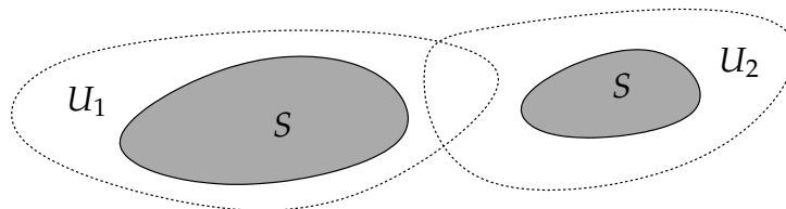
Figure 7.7: Disconnected subset. Notice that U_1 \cap U_2 need not be empty, but U_1 \cap U_2 \cap S = \emptyset .
