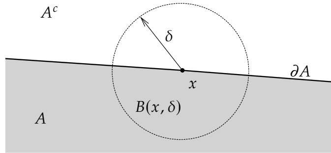
Figure 7.9: Boundary is the set where every ball contains points in the set and also its complement.
