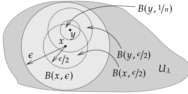
Figure 7.12: Proof of Lebesgue covering lemma. Note that B(y, \epsilon/2) \subset B(x, \epsilon) by triangle inequality.
