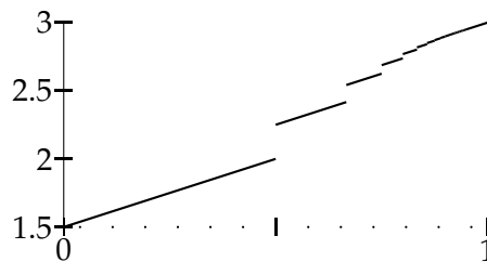
Figure 3.12: Strictly increasing function on [0, 1] with countably many discontinuities.
