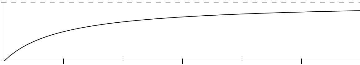
Figure 7.2: Graph of \frac{t}{t+1} for positive t with an asymptote at 1.
