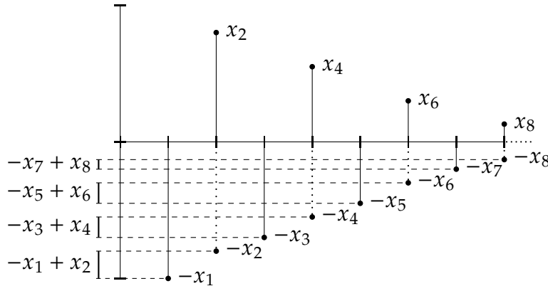
Figure 2.8: Showing that 0 \geq s_{2k} \geq -x_1 where k = 4 for an alternating series.
