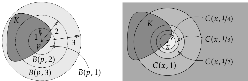
Figure 7.11: Proving compact set is bounded (left) and closed (right).
