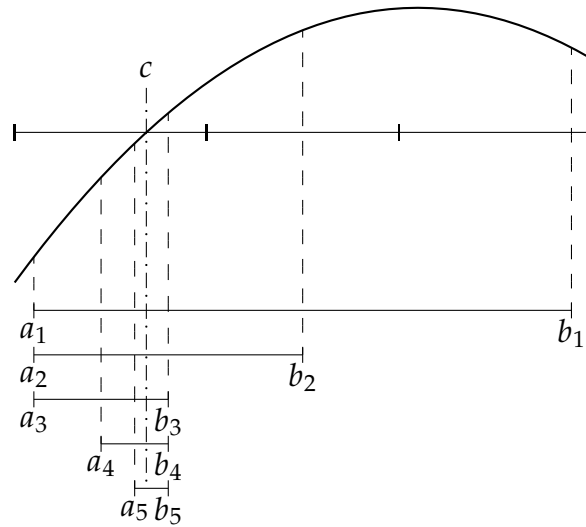
Figure 3.7: Finding roots (bisection method).
