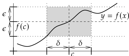
Figure 3.3: For |x - c| < \delta , the graph of f(x) should be within the gray region.
