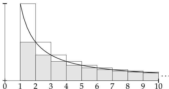
Figure 5.10: The area under the curve, \int_1^\infty f , is bounded below by the area of the shaded rectangles, f(2) + f(3) + f(4) + \cdots , and bounded above by the area entire rectangles, f(1) + f(2) + f(3) + \cdots .
