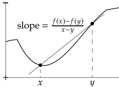
Figure 3.9: The slope of a secant line. A function is Lipschitz if \left| \frac{f(x)-f(y)}{x-y} \right| \leq K for all x and y .
