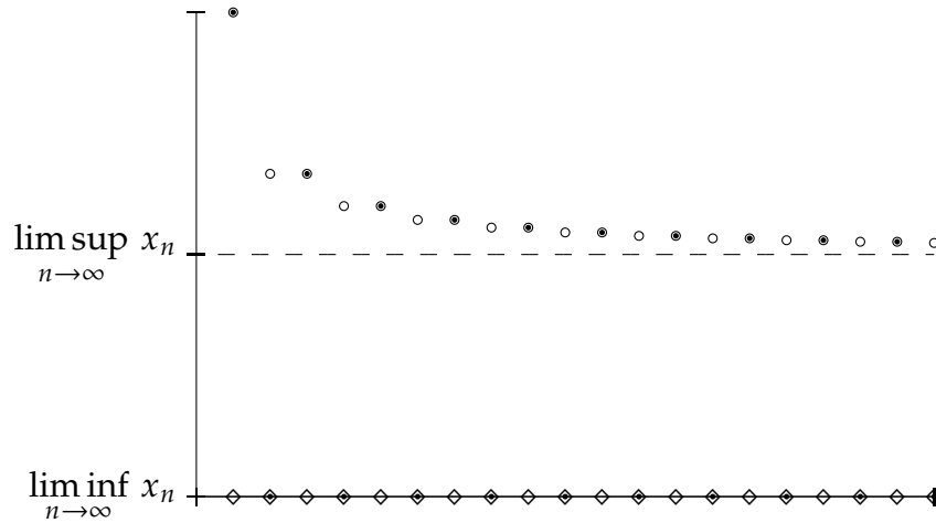
Figure 2.6: First 20 terms of the sequence in Example 2.3.3 . The marking is as in Figure 2.5 .
