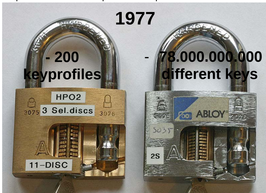
Two High security padlocks from the 70's.
