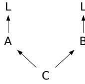
Figure 4: Non-virtual base [fig:class.nonvirt]
