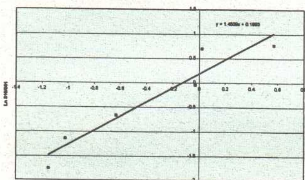
Graph 2. Item difficulty difference versus linear transformation of Ln S_{10}/S_{01}
