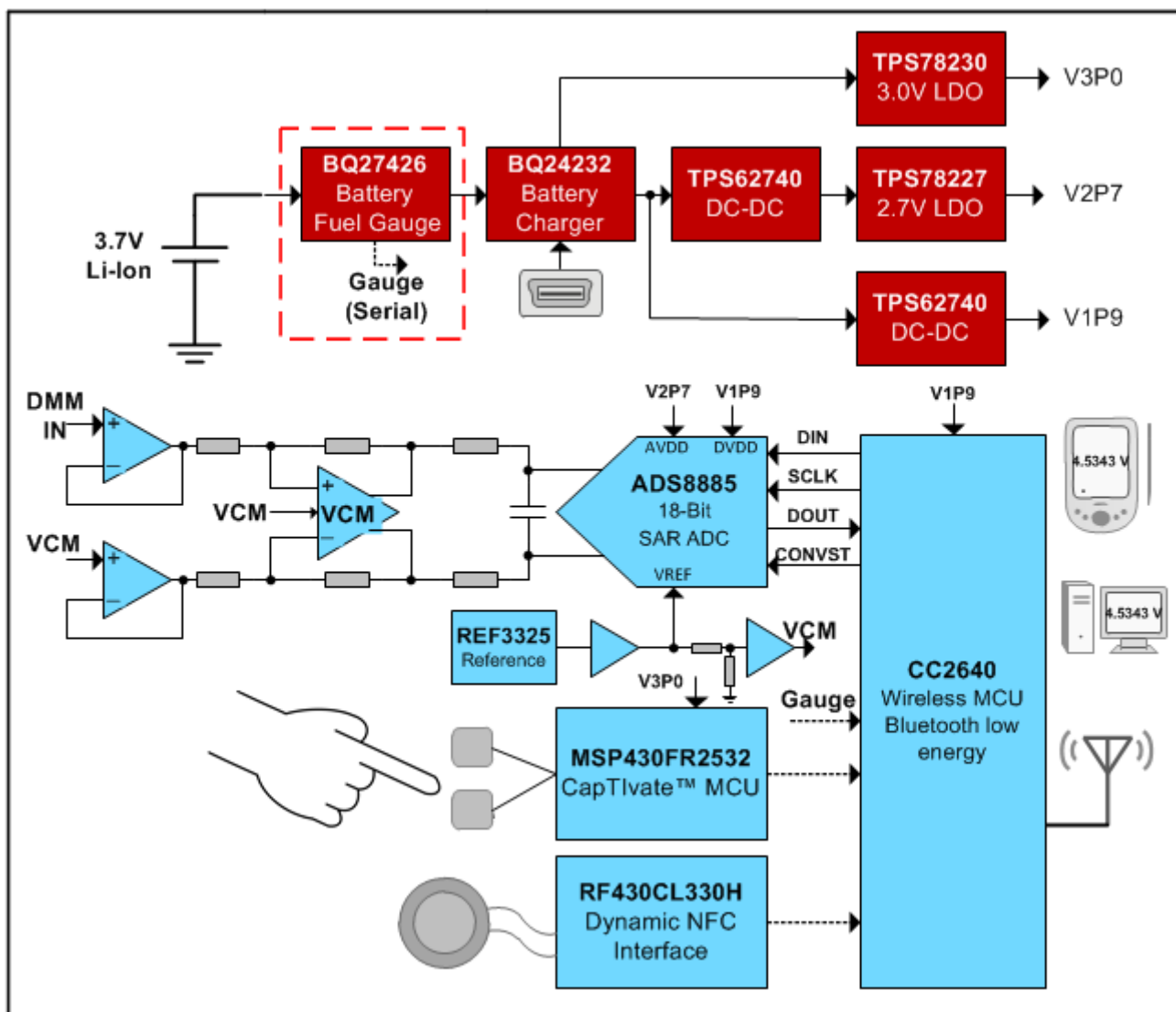
Figure 1. Wireless DMM Block Diagram
