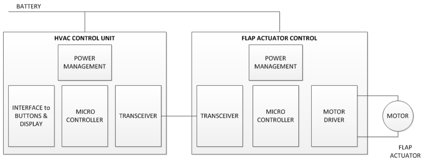
Figure 2. Remote Control of Flap Actuator Motor
