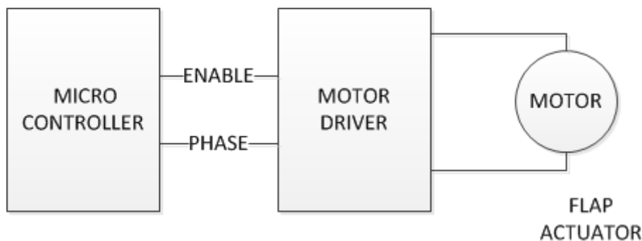
Figure 5. A Microcontroller Controlling the Motor Driver Directly
