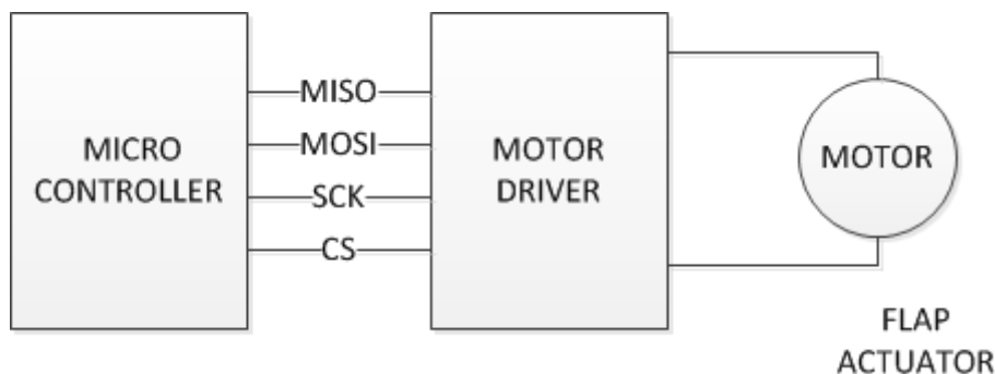
Figure 4. A Microcontroller Communicating with the Motor Driver Using SPI
