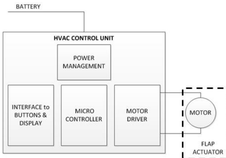
Figure 3. Integrated Motor Driver for Flap Actuator
