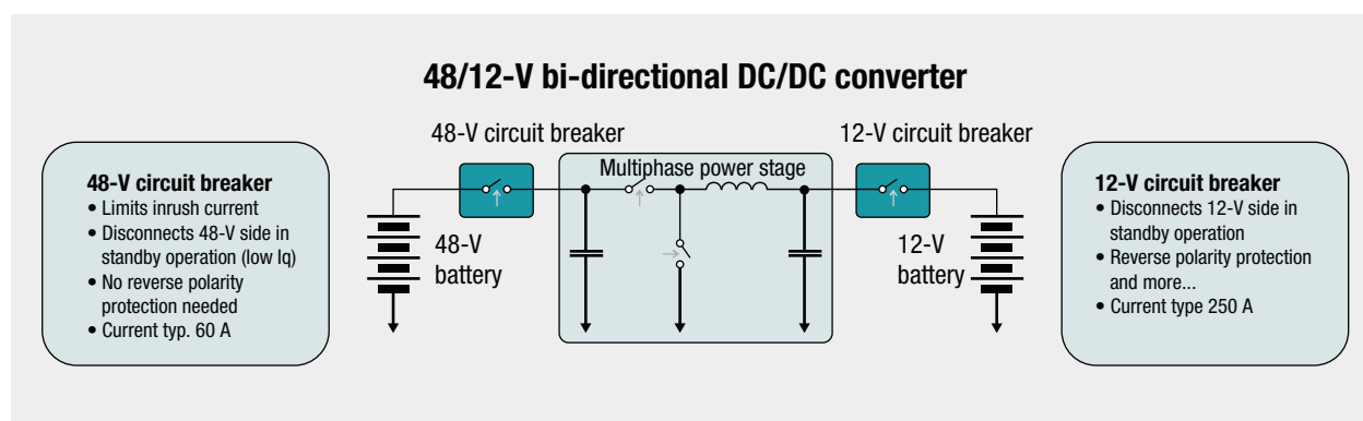
Figure 2. 48/12-V bidirectional DC/DC converter.
