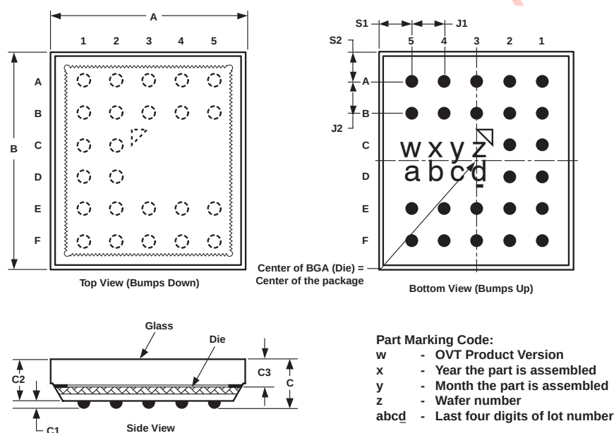
Figure 13 OV7670/OV7171 Package Specifications
