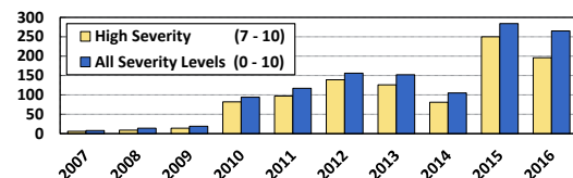
Figure 1: Use-after-free vulnerabilities in NVD [48].
