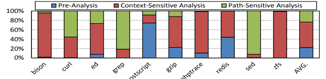
Figure 11: Percentage distribution of CRED's analysis times.
