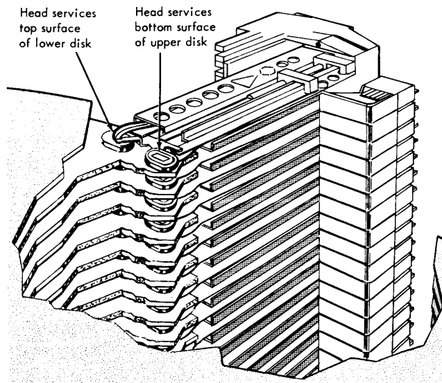
Figure 2. Head Arrangement
