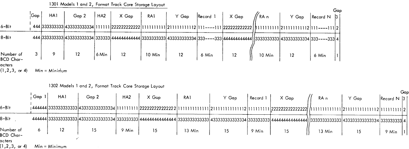
Figure 8. Core Storage Format Control Record — n Records
