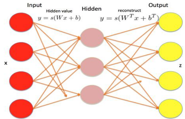
Fig 1: Denoising auto-encoder
