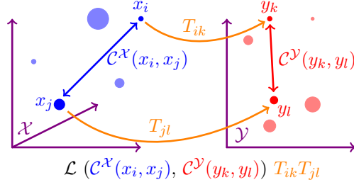
Fig. 1: Illustration of GW, with only one term L_{ijkl} of the quadruple sum of Eq. (5).
