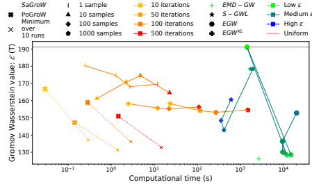
Fig. 19: Similar to the Figures 7, 8 and 9 in the paper, with \text{SaGroW}^{KL} replaced by \text{SaGroW} .
