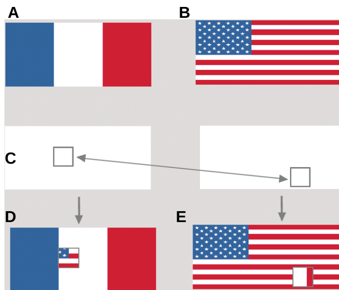
Fig. 2. Wolpert's concept of a universal positional field, illustrated with his French Flag Model. The white rectangles, and the rectangles bounding the flags, represent positional fields; two different genotypes (fr and us) give rise to the patterns (phenotypes) in (A,B), respectively. If reciprocal tissue transplants (C) are made at an early stage between the two species, the transplanted cells are predicted to develop according to their own genome and developmental history, but to read the positional information in the host positional field. Thus they develop as an island of donor-type pattern that is appropriate to the host positional information (D,E). Based on Fig. 5 in (Wolpert, 1969).
