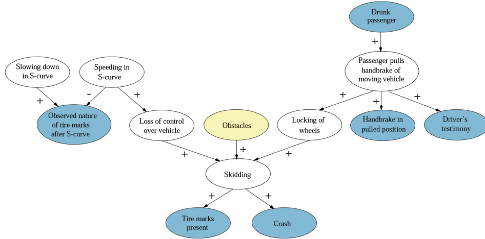
Figure 2: Causal structure for the case.
