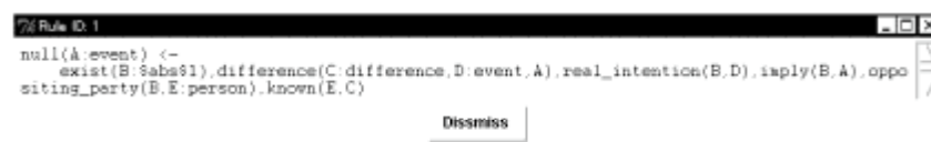
Figure 4.12. The hypothetical rule
