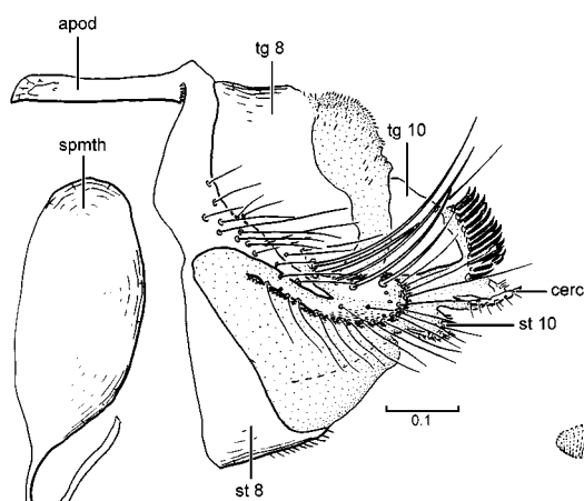
235. Sabroskyella rancheria
