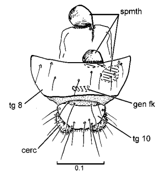
248. Microsania sp.
