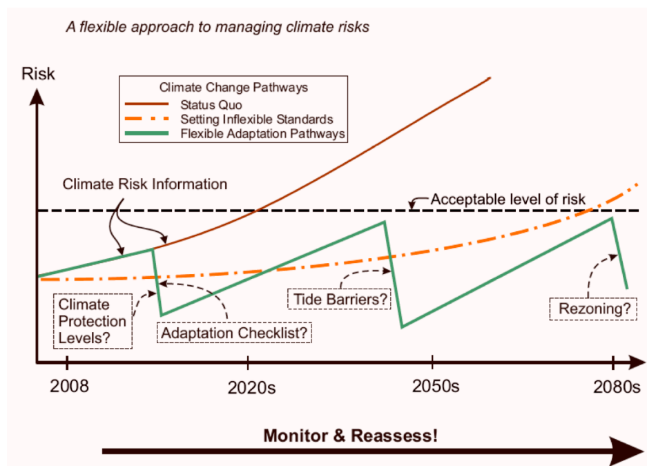
Figure 7. Generic illustration of flexibly staged, multiple decision paths for adaptation measures to manage rising risks related to climate change. Note that timing and actions are hypothetical examples only and do not imply recommendations for real actions. For details see text. (Source: CCSR of Columbia University)
