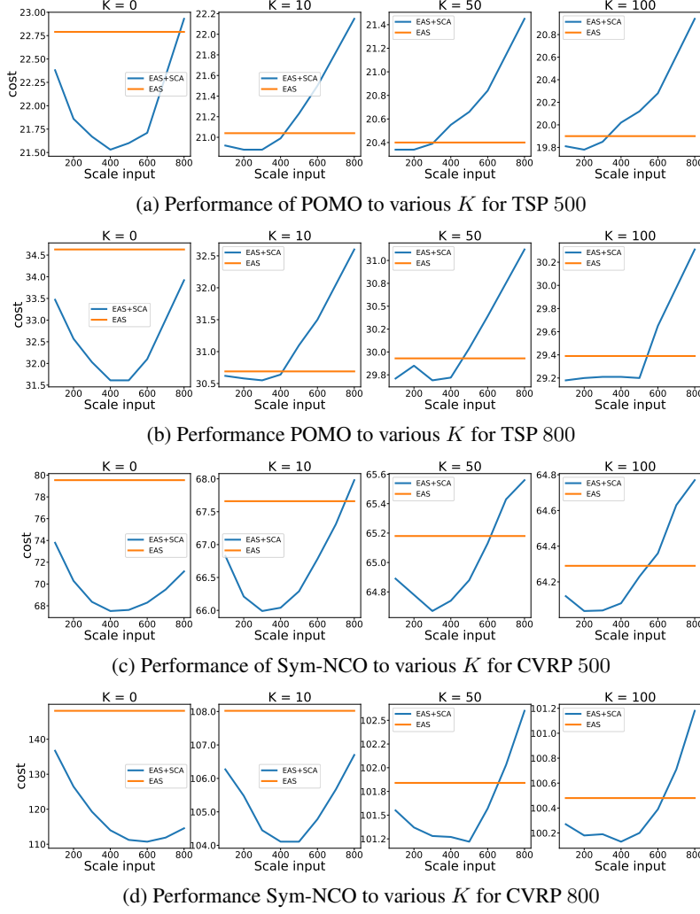
Figure 5: The few-shot performance for various K of TSP and CVRP.
