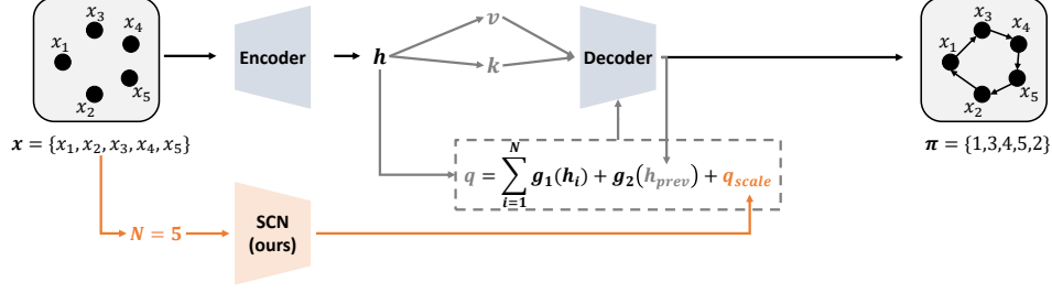
Figure 1: The scale conditioned network combined with DRL model for combinatorial optimization.
