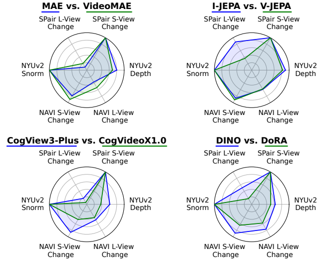
Figure 1. The diashow paradox. Streamlining the evaluation protocol, we develop AnyProbe , a framework to systematically compare video and image models on depth, surface normals (NYUv2 [26]), and multi-view correspondences [18, 23]. Contrary to a common-sense expectation, we find that video-based vision foundation models (green) do not provide a consistent advantage over image-based models (blue) on 3D awareness tasks.
