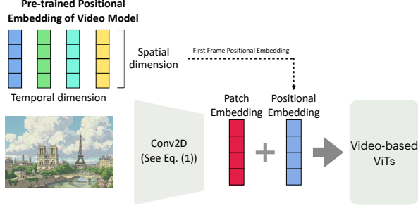
Figure 2. Adapting video-based ViT models for image tasks. We tokenize the image using a 2D patch-embedding convolution adapted for the video model (Eq. (1)), as in image ViTs, and use only the spatial positional embeddings of the first frame.
