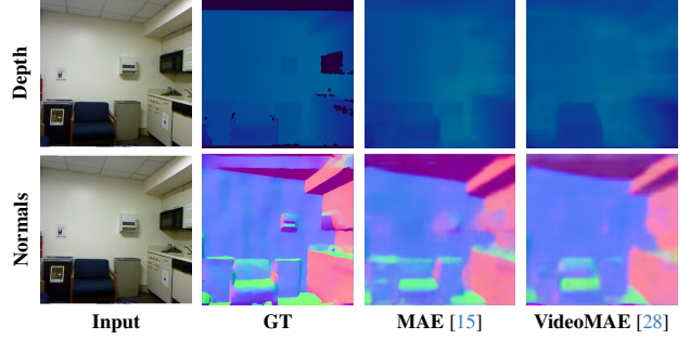
Figure 3. Qualitative examples. We visualize depth and surface normal maps derived from running AnyProbe with a DPT [36] head on frozen MAE and VideoMAE on NYUv2 [26]. MAE produces consistently sharper, more accurate geometry.
