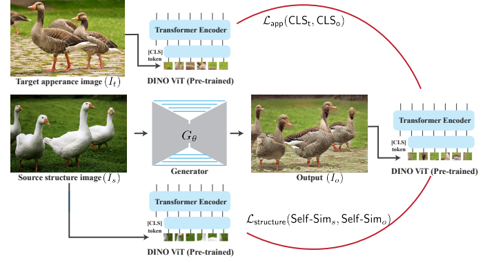
Fig. 2. Splice pipeline. Our generator G_\theta takes an input structure image I_s and outputs I_o . We establish our training losses using a pre-trained and fixed DINO-ViT model, which serves as an external semantic prior: we represent structure via the self-similarity of keys in the deepest attention module (Self-Sim), and appearance via the [CLS] token in the deepest layer. Our objective is twofold: (i) \mathcal{L}_{app} encourages the [CLS] of I_o to match the [CLS] of I_t , and (ii) \mathcal{L}_{structure} encourages the self-similarity representation of I_o and I_s to be the same. See Sec. 3.3 for details.
