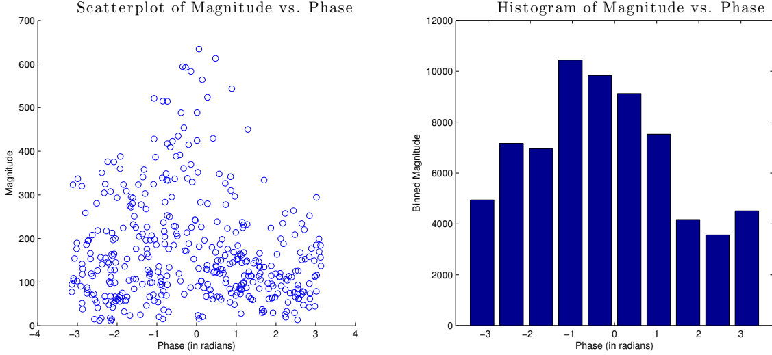
Figure 4.2: Plotting the magnitude of the composite signal against the phase of the composite signal, we recover a compelling visual of the nonuniformity (and hence noncircularity) of the composite signal y[n]
