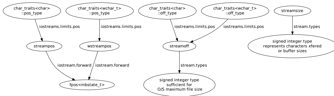
Figure 6 — Stream position, offset, and size types [non-normative]
