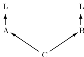
Figure 3 — Non-virtual base
