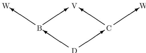
Figure 6 — Name lookup
