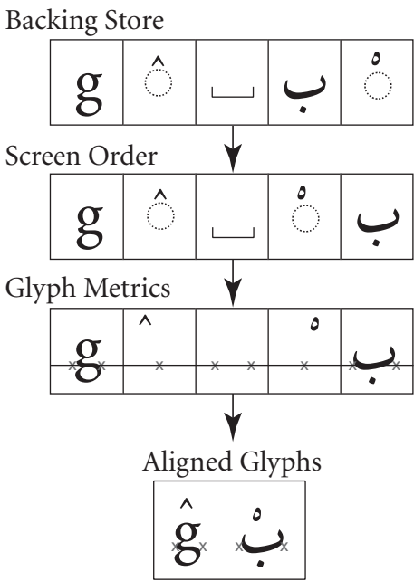
Figure 5-8. Bidirectional Placement
