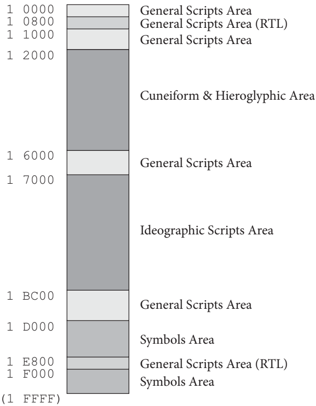
Figure 2-15. Allocation on Plane 1
