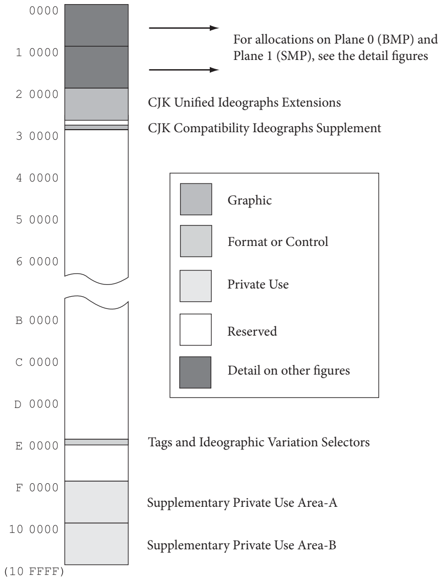
Figure 2-13. Unicode Allocation
