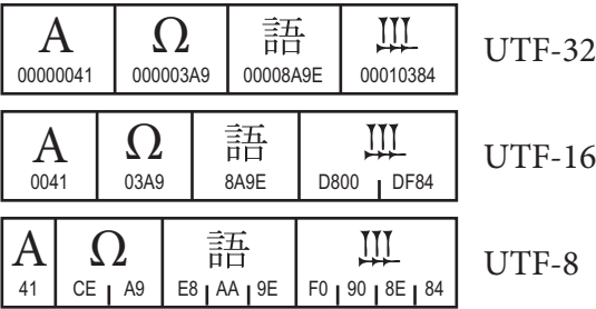
Figure 2-11. Unicode Encoding Forms
