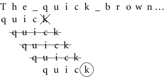
Figure 5-13. Sublinear Searching
