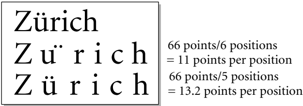
Figure 5-9. Justification
