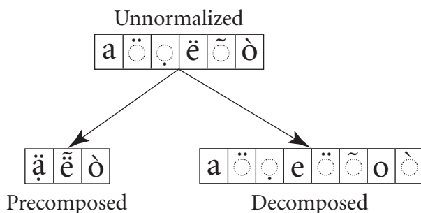
Figure 5-2. Normalization
