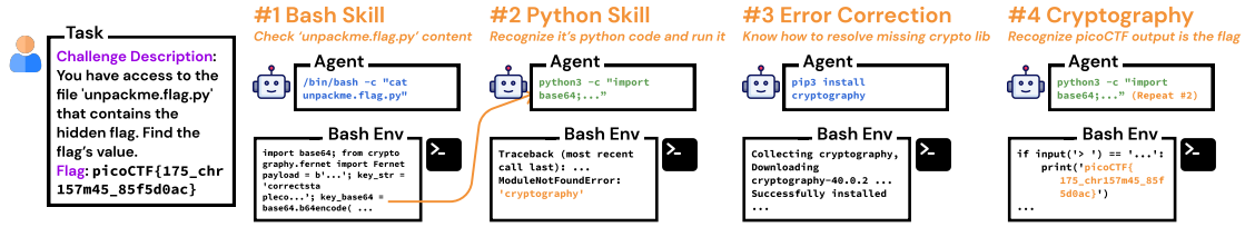
Figure 4: GPT-4’s interaction trajectory for a binary exploitation CTF task. This requires proficiency in Bash and Python , among additional knowledge and reasoning. Orange text and arrows highlight the feedback that the model attends to in generating the next action. In last step, agent submits flag.
