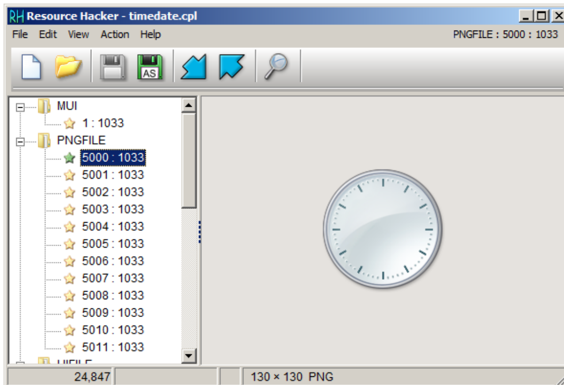
Fig. 8.10: Resource Hacker
