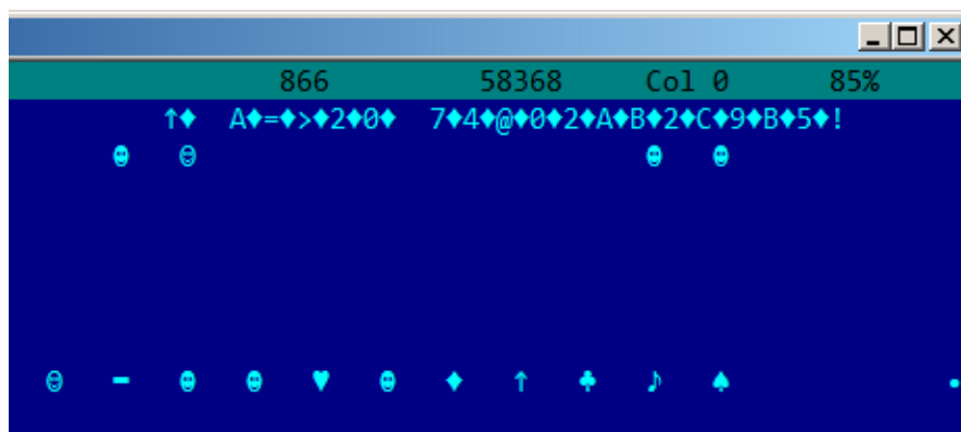
Fig. 5.5: Hiew: UTF-16LE
