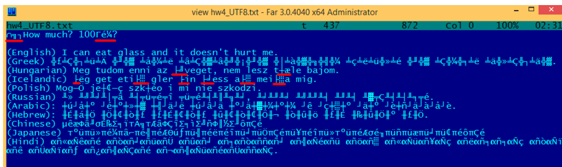
Fig. 5.2: FAR: UTF-8
