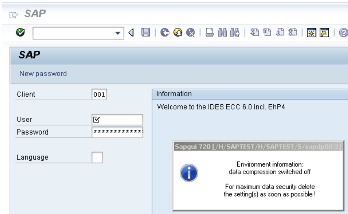
Fig. 8.17: Screenshot
