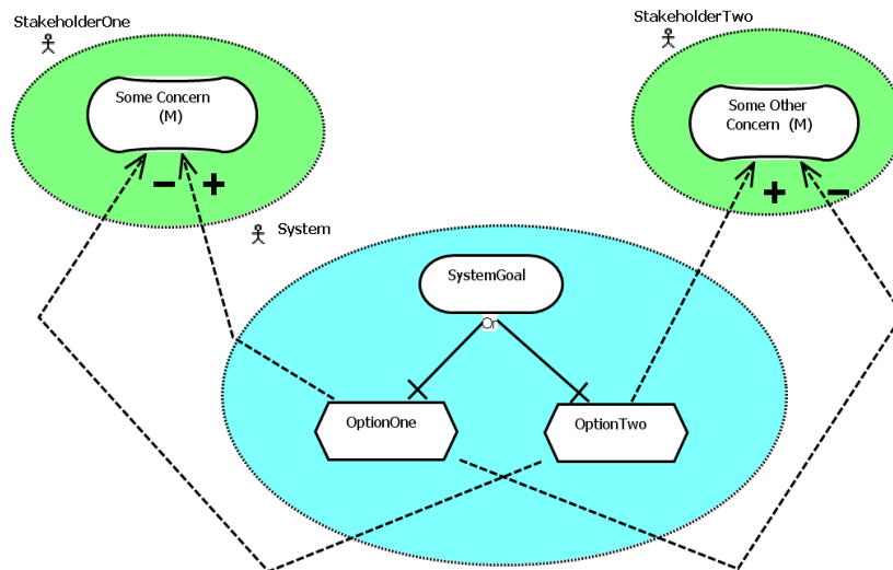
Fig. 1. Common GRL pattern for decision making in context
