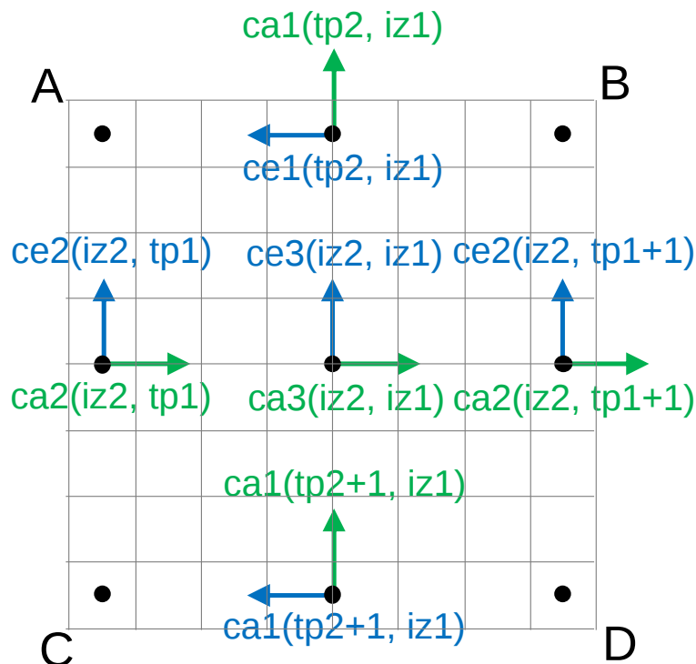
Figure J.5. The parametric representation of the interpolation coefficients cea = (ce, ca) , stored in the interpolation parameters ce1 , ca1 , ce2 , ca2 , ce3 and ca3 , is equivalent to five additional tie points for the interpolation subarea. Shown with parameter orientation and indices.
