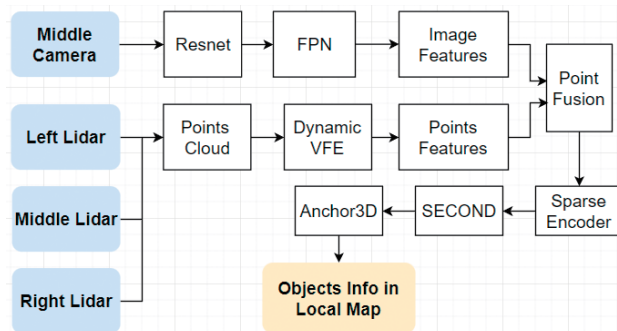
Figure 3 Structure of deep learning based neural network
