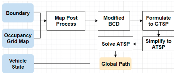
Figure 6 Exploration planner
