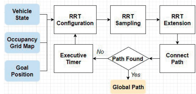
Figure 7 Sweeping planner
