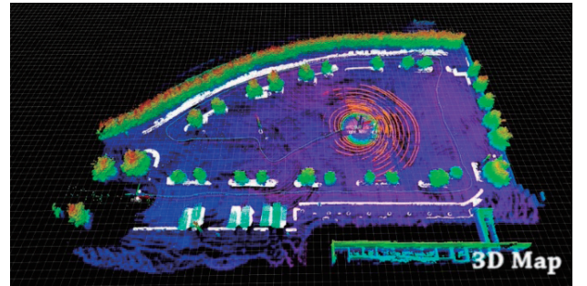
Figure 10 3D Map
