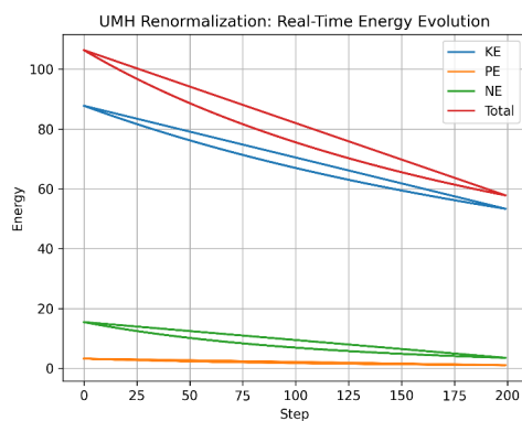
Figure 148: RESULT: Time evolution of energy components across grid resolutions. Consistent decay rates confirm renormalization stability.
