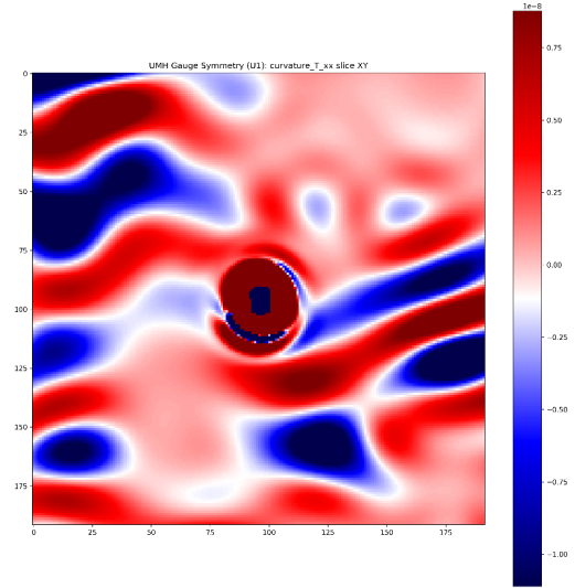
Figure 95: RESULT: U(1) phase-lock — curvature \nabla^2 T_{xx} . Corresponding curvature remains smooth and isotropic under local U(1) constraint.
