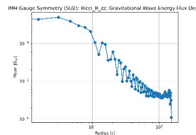
Figure 140: Radial decay of |R_{zz}| . Matched falloff with G_{zz} confirms consistency between curvature and stress-energy balance.
