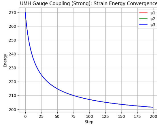
Figure 127: RESULT: Strong SU(3) Energy Convergence. Strain energy decreases over relaxation steps, suggesting a stabilized SU(3) gauge-like phase entanglement in the UMH framework.
