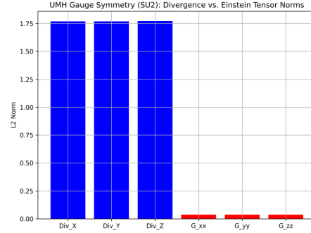
Figure 135: RESULT: UMH gauge symmetry (SU(2)). L^2 norms of Einstein-tensor components ( G_{xx}, G_{yy}, G_{zz} ) and of the covariant divergence \nabla_\mu G^{\mu\nu} . Across the domain, \|\nabla_\mu G^{\mu\nu}\| \ll \|G_{\mu\nu}\| (Bianchi consistency). Outside core regions (no dominant sources), \|G_{\mu\nu}\| is itself small, indicating approximate vacuum.
