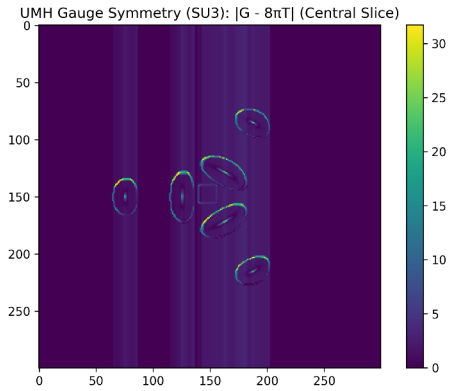
Figure 68: RESULT: UMH Gauge Symmetry (SU3): Residual magnitude field |G_{\mu\nu} - \frac{8\pi G}{c^4} T_{\mu\nu}| . Residuals remain negligible across most of the lattice and are localized to dynamic core regions, validating numerical consistency with Einstein's equations.
