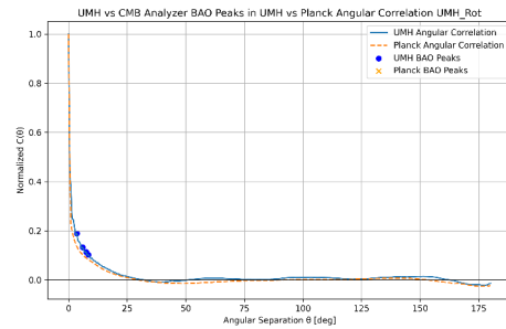
Figure 75: RESULT: BAO peak analysis comparing UMH angular correlation with Planck data. UMH spectrum shows naturally emerging BAO-like structures without requiring any injected oscillations.
