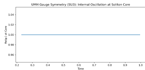
Figure 112: RESULT: Soliton core confinement — field oscillation. Real part of \psi_1 at the soliton core remains phase-locked and constant.
