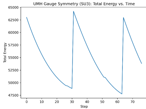
Figure 115: RESULT: Gauge field evolution — total energy. Total system energy shows periodic modulation from breathing mode cycling.
