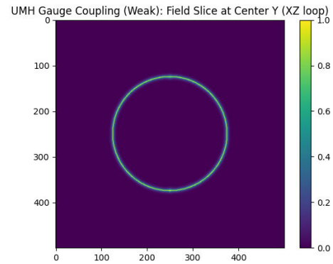
Figure 124: RESULT: SU(2) Field Slice (XZ loop). Phase loop initialized in the XZ plane. Field superposition and tension locking emulate weak-force phase constraints.
