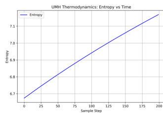
Figure 150: RESULT: Entropy vs time. Entropy increases and stabilizes, signaling approach to equilibrium.
