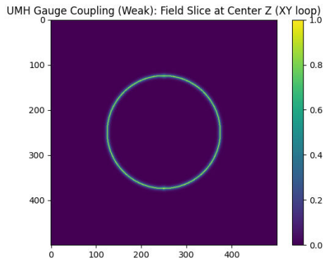
Figure 123: RESULT: SU(2) Field Slice (XY loop). Phase loop initialized in the XY plane. Field superposition and tension locking emulate weak-force phase constraints.
