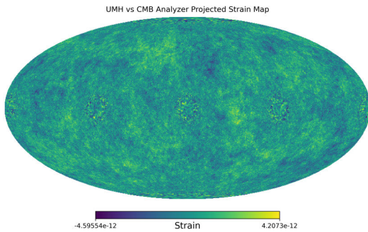
Figure 74: RESULT: Projected UMH strain map after HEALPix projection, showing isotropy and structural coherence similar to observed CMB sky maps.
