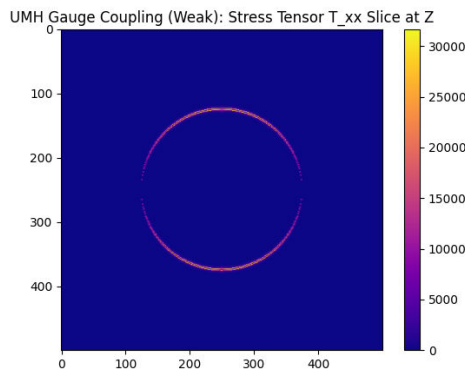
Figure 125: RESULT: Weak-coupling stress component T_{xx} . Ring-localized normal stress from SU(2)-locked field gradients.
