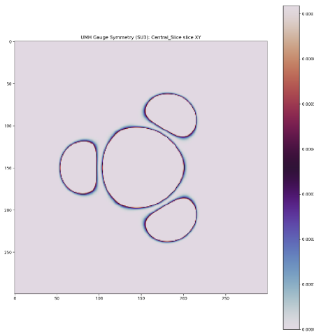
Figure 117: RESULT: SU(3) wavefield topology — central slice. Central slice of wavefield amplitude confirms strong solitonic localization.
