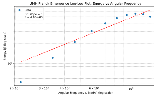
Figure 54: RESULT: Log-log plot of E vs. \omega , confirming a power-law relation with slope \approx 1 .
