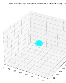
Figure 46: RESULT: 3D isosurface midway through propagation.
