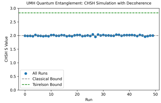
Figure 131: RESULT: Per-run CHSH S (same N = 50 baseline). Reference lines at S = 2 and 2\sqrt{2} . In the independent baseline no points exceed Tsirelson; “UMH-tagged” annotations appear only when the diagnostic relaxed-independence mode is enabled.
