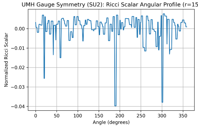
Figure 143: RESULT: SU(2) Ricci scalar R angular profile at radius r = 15 . The distribution remains nearly isotropic with low-amplitude angular noise and narrow dips ( < 4\% ), likely arising from internal oscillations or boundary reflections.
