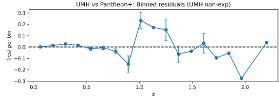
Figure 81: RESULT: Binned residual means with standard errors. Points fluctuate about zero across the full redshift range.
