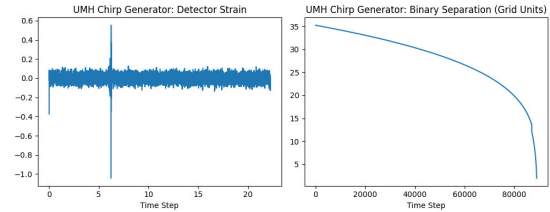
Figure 60: RESULT: UMH Chirp Generator: Dynamic preview at Hanford. Left: Simulated detector strain showing transient chirp structure consistent with a coalescing binary waveform. Right: Corresponding binary separation in grid units, decreasing monotonically toward merger.
