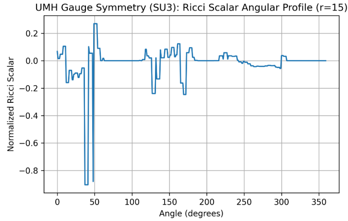
Figure 144: RESULT: SU(3) Ricci scalar angular distribution sampled at fixed radius. Despite strong internal gradients, the angular Ricci profile remains centered near zero with no large-scale asymmetries.
