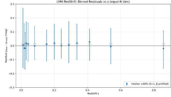
Figure 88: RESULT: Equal- N binned residuals. Median \pm 68\% intervals per redshift bin; medians fluctuate around zero across the full range.
