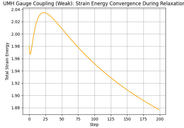
Figure 122: RESULT: Weak SU(2) Energy Convergence. Relaxation of strain energy during the SU(2) test confirms stable tension transfer between the crossed loops. The final energy is used to estimate the effective weak coupling constant.
