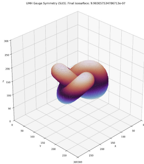
Figure 102: RESULT: SU(3) field topology — 3D isosurface. Final \psi field showing preserved trefoil structure.
