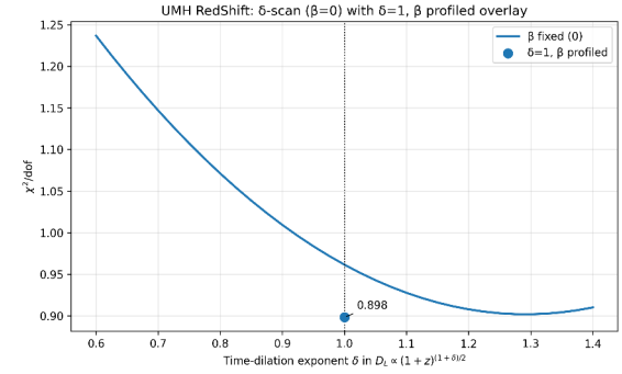
Figure 90: RESULT: \chi^2/\text{dof} vs. \delta (diagnostic). With \beta fixed to 0 (solid), the minimum lies near \delta \approx 1.30 . The preferred point ( \delta = 1 , \beta profiled; dot) sits in the same trough with \chi^2/\text{dof} \approx 0.898 .
