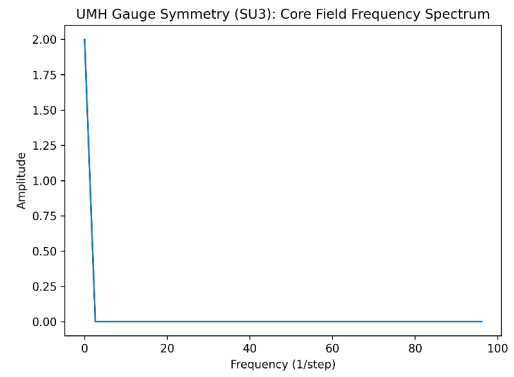
Figure 114: RESULT: Soliton core confinement — FFT analysis. Frequency spectrum confirms harmonic mode confinement and absence of noise-induced broadening.
