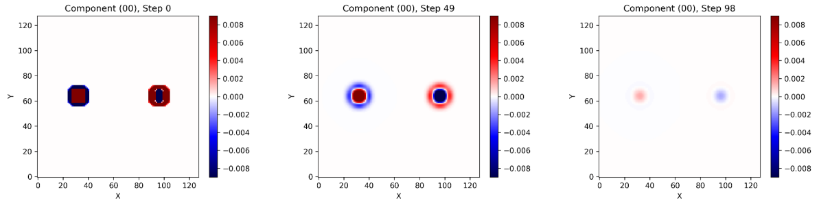
RESULT: UMH MultiBody GW Ricci Frame 000
