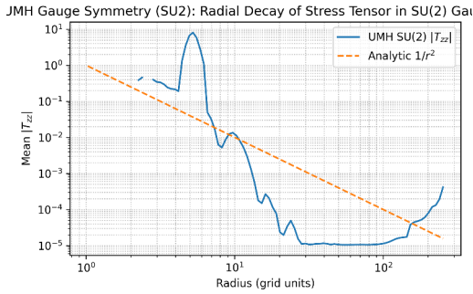
Figure 134: RESULT: UMH Gauge Symmetry (SU2): Radial decay of the stress tensor component T_{zz} measured from the soliton center. The numerical profile approximately follows an inverse-square scaling ( \propto 1/r^2 ), consistent with the expected Newtonian-limit behavior of gravitational stress propagation in the ultronic medium.
