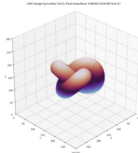
Figure 118: RESULT: SU(3) wavefield topology — 3D structure. Final isosurface reveals a trefoil-knot-like solitonic structure preserved through constraint dynamics.
