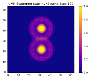
RESULT: Step 120: Overlap intensifies as bosons merge transiently under coherent phase locking.
