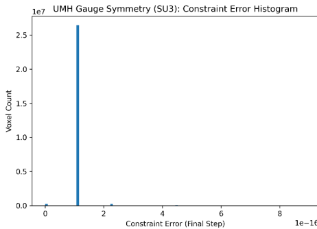
Figure 111: RESULT: Constraint validation — error histogram. Distribution of constraint errors across all voxels at the final simulation step.
