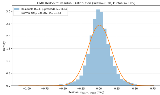
Figure 89: RESULT: Residual distribution. Histogram of \mu_{\text{data}} - \mu_{\text{UMH}} with normal fit: mean \approx 0.007 mag, width \sigma \approx 0.163 mag (mild skew -0.28 , kurtosis 3.85 ).
