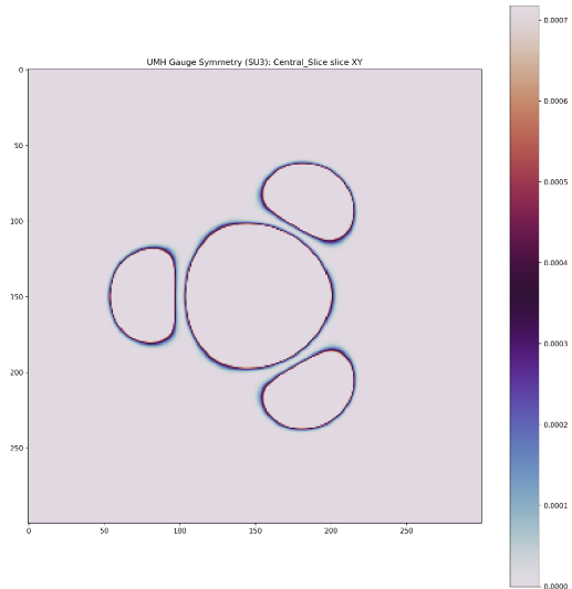
Figure 103: RESULT: SU(3) field topology — central slice. Central slice showing symmetric confinement.
