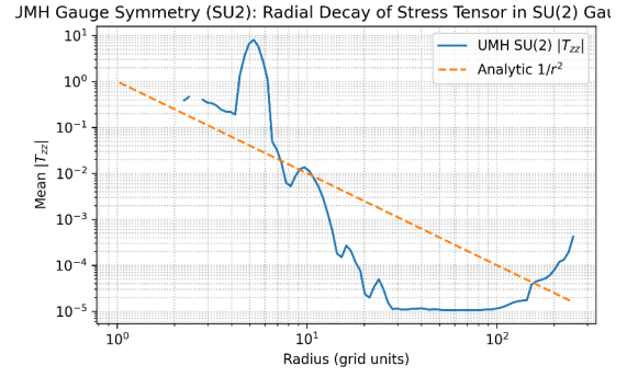
Figure 64: RESULT: UMH Gauge Symmetry (SU2): Radial profile of |T_{zz}| from the soliton center, compared to the analytic 1/r^2 decay. The profile exhibits approximate power-law behavior consistent with Newtonian-limit gravitational scaling over intermediate distances.
