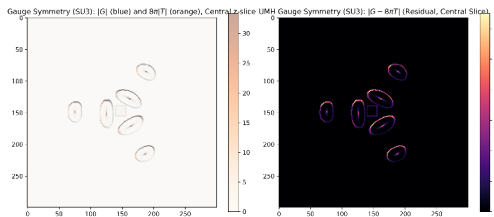
Figure 109: RESULT: SU(3) gauge dynamics — G vs. T comparison. Central slice showing |G| and 8\pi|T| for G_{zz} and T_{zz} components, demonstrating tight agreement.
