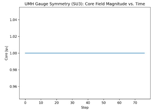
Figure 116: RESULT: Gauge field evolution — core field stability. Field magnitude at the soliton core remains stable throughout the simulation.
