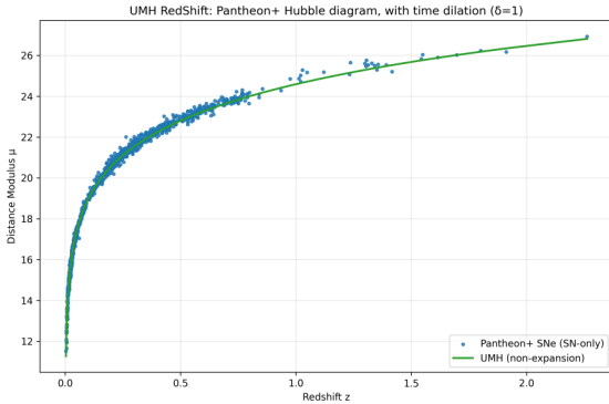
Figure 85: RESULT: Pantheon+ Hubble diagram (UMH, \delta = 1 ). SN-only sample ( N = 1624 ) with the UMH non-expansion curve using a^* = \alpha and profiled \beta ; M profiled analytically (full STAT+SYS GLS).
