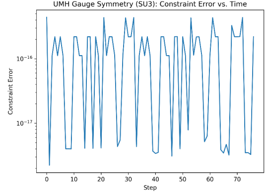
Figure 99: RESULT: SU(3) constraint error — vs. time. Maximum constraint error remains within machine precision.
