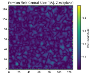
Figure 91: RESULT: Fermionic spatial soliton separation (exclusion behavior).
