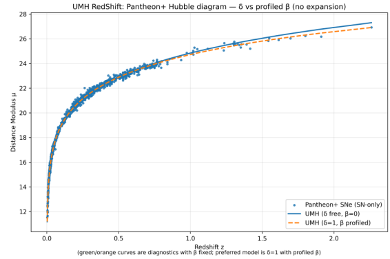
Figure 86: RESULT: \delta vs. profiled \beta (diagnostic). Comparison of the diagnostic case with \delta free, \beta = 0 (solid) and the preferred case \delta = 1 with \beta profiled (dashed). The preferred curve tracks the data at high z .
