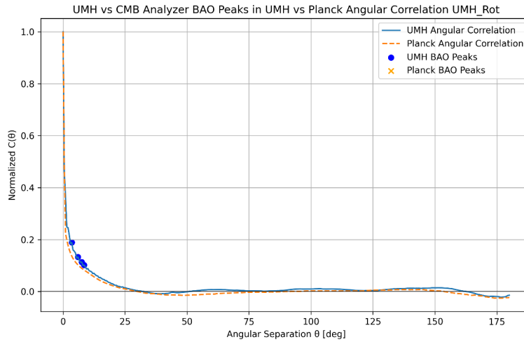
Figure 77: RESULT: BAO peak comparison between UMH angular correlation and Planck data after rotation. Multiple peaks emerged naturally, matching known BAO scales without artificial tuning.
