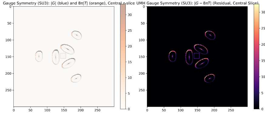
Figure 66: RESULT: UMH Gauge Symmetry (SU3): Central slice comparing Einstein tensor G_{\mu\nu} and stress-energy tensor T_{\mu\nu} , with overlays marking soliton core regions. Spatial agreement confirms G_{\mu\nu} = \frac{8\pi G}{c^4} T_{\mu\nu} near peak energy densities.
