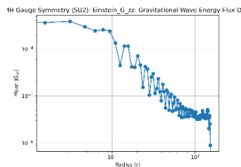
Figure 139: Radial decay of |G_{zz}| . Mean magnitude versus radius confirms near-zero divergence outside dynamic core, validating conservation.
