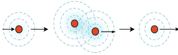
Figure 159: Mechanical Scattering of Solitons. Soliton interactions in the ultronic medium occur via nonlinear strain overlap. The sequence shows approach, interference, deflection, and separation — providing a mechanical analog to quantum scattering without virtual particles.
