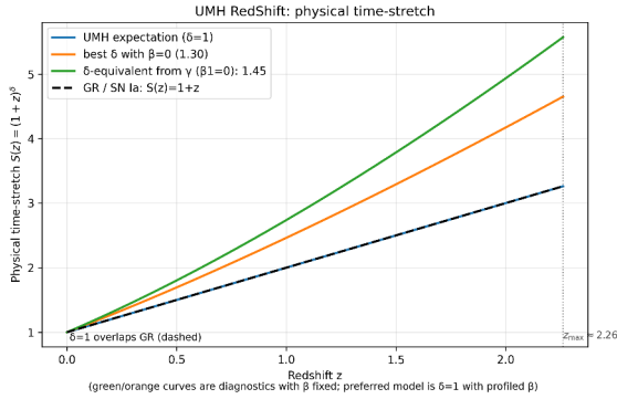
Figure 154: RESULT: Cosmological time stretch in UMH. The time-stretch factor S(z) = (1 + z)^\delta . The preferred setting \delta = 1 (adopted in the Hubble-diagram fits) coincides with the SN Ia stretch relation; diagnostic \delta scans are discussed in the text.
