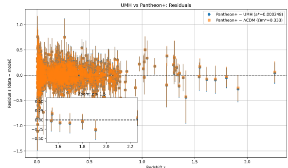
Figure 79: RESULT: High- z residuals (zoom): no systematic bias; both models track the data within uncertainties.
