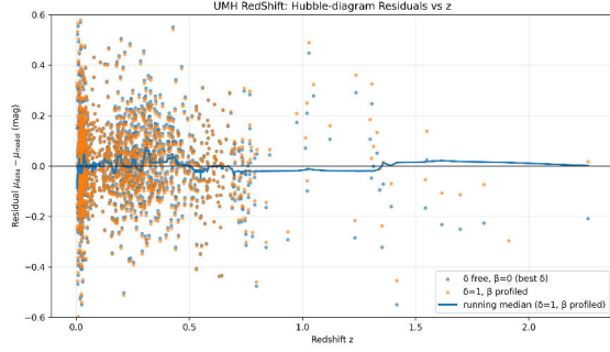
Figure 87: RESULT: Residuals vs. z (mag). \mu_{\text{data}} - \mu_{\text{UMH}} ; running median (blue) stays near zero with no visible drift. Unweighted slope(residual vs. z ) \approx 0 .
