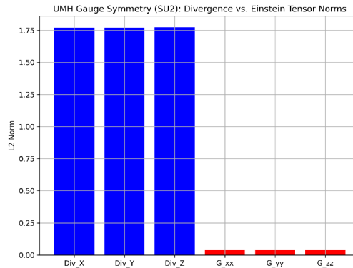
Figure 65: RESULT: UMH gauge symmetry (SU(2)). L^2 norms of Einstein-tensor components ( G_{xx}, G_{yy}, G_{zz} ) and of the covariant divergence \nabla_\mu G^{\mu\nu} . Across the domain, \|\nabla_\mu G^{\mu\nu}\| \ll \|G_{\mu\nu}\| (Bianchi consistency). Outside core regions (no dominant sources), \|G_{\mu\nu}\| is itself small, indicating approximate vacuum.
