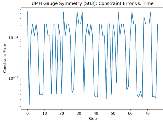
Figure 113: RESULT: Constraint validation — error vs. time. Evolution of maximum constraint error showing machine-level stability.
