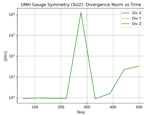
Figure 106: RESULT: SU(2) gauge field — divergence norm. Norm of \nabla^\mu T_{\mu\nu} decays over time, validating conservation.
