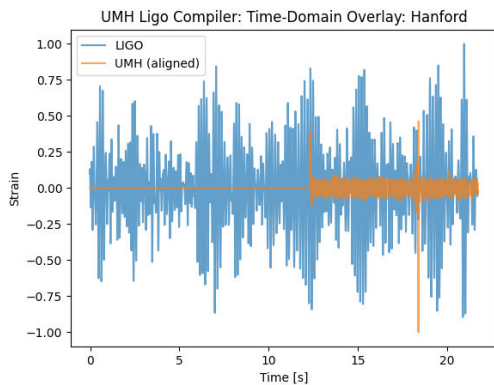
Figure 61: RESULT: UMH – LIGO time-domain overlay at Hanford. Comparison between the observed LIGO strain signal (blue) and the UMH-aligned synthetic waveform (orange). The temporal and amplitude alignment illustrate close correspondence in the chirp region, validating waveform phase consistency.
