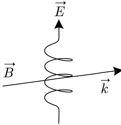
Figure 157: Right-handed transverse strain wave in the ultronic medium. The electric-like displacement \vec{E} is perpendicular to both the magnetic-like rotational strain \vec{B} and the direction of wave propagation \vec{k} . The chirality is enforced by the phase rotation and mechanical tension constraints of the medium.
