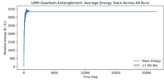
Figure 133: RESULT: Mean relative energy vs. timestep across runs (shaded \pm 1\sigma ). The trace indicates numerical stability/conservation during the entanglement simulations.
