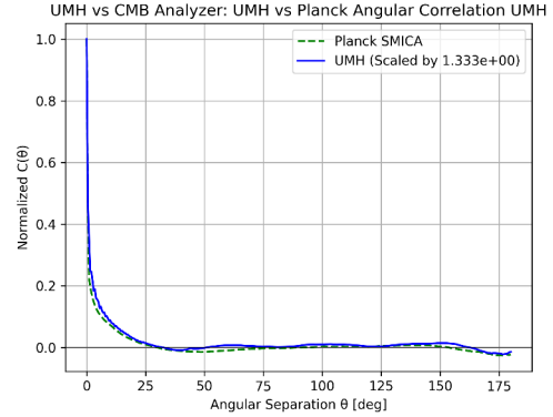
Figure 73: RESULT: UMH vs. Planck angular correlation C(\theta) , showing matching behavior especially near \theta = 155^\circ , validating the emergent horizon scale from UMH dynamics.
