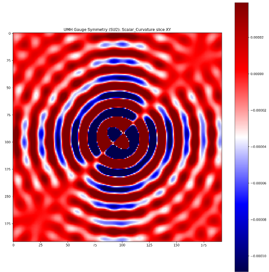
Figure 97: RESULT: SU(2) constraint — scalar curvature slice. Confirms coherent solitonic curvature generation.
