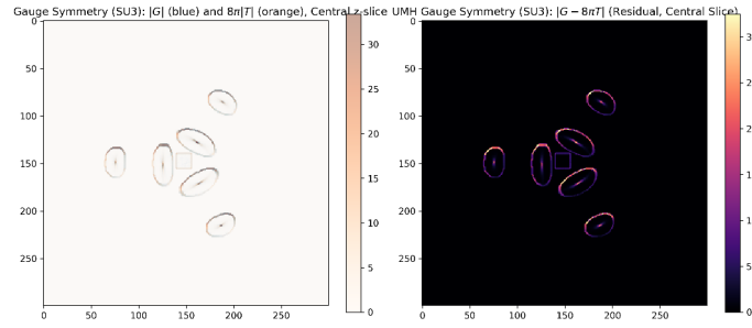
Figure 136: RESULT: UMH Gauge Symmetry (SU3): Overlaid spatial comparison of G_{\mu\nu} and T_{\mu\nu} fields. Peak locations are co-spatial, validating strong-field agreement. Colored circles mark regions of maximum curvature and mass-energy.
