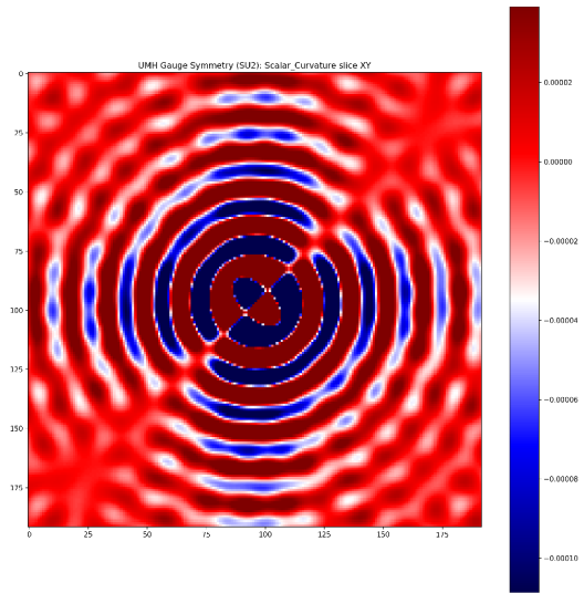
Figure 107: RESULT: SU(2) gauge field — scalar curvature slice. Scalar curvature aligned with the soliton center.
