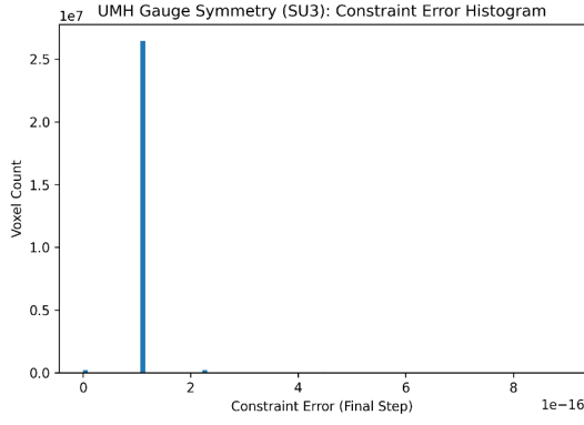
Figure 98: RESULT: SU(3) constraint error — histogram. Distribution of constraint errors at final step.
