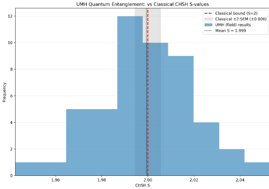
Figure 132: UMH baseline S -distribution overlaid on a classical reference band ( 2 \pm 2 \cdot \text{SEM} , gray). The observed sample falls within the band, consistent with the classical bound under measurement independence.
