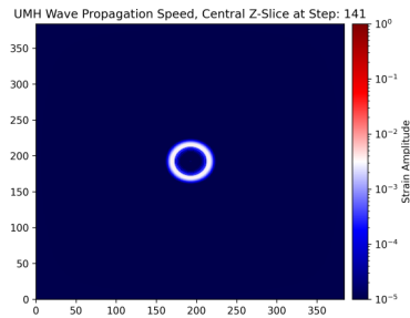
Figure 43: RESULT: Mid-evolution slice showing smooth outward propagation.
