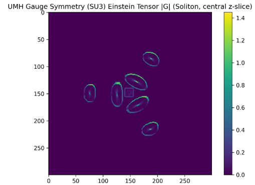
Figure 110: RESULT: SU(3) gauge dynamics — Einstein tensor. Magnitude of the Einstein tensor for the solitonic configuration.
