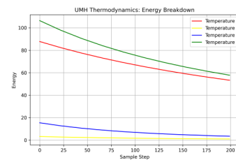
Figure 152: RESULT: Evolution of energy components: kinetic, potential, and nonlinear.
