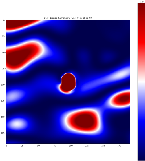
Figure 94: RESULT: U(1) phase-lock — T_{xx} stress slice. T_{xx} slice from a phase-locked soliton.
