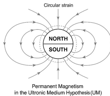
Figure 158: Persistent magnetic field formation in the Ultronic Medium Hypothesis (UMH). A solitonic phase-coherent domain generates a circulating rotational strain pattern in the surrounding medium, producing a stable magnetic field. The arrows represent the mechanical strain curvature lines, which emerge from the North pole and re-enter at the South pole, consistent with classical magnetic dipole behavior. The dashed circle indicates the locked circular strain boundary, maintained by soliton alignment.
