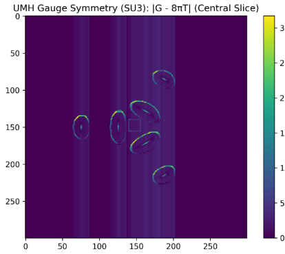
Figure 137: RESULT: UMH Gauge Symmetry (SU3): Residual field |G_{\mu\nu} - 8\pi T_{\mu\nu}| computed across the domain. Residuals remain negligible outside the soliton core, supporting UMH's consistency with general relativity.
