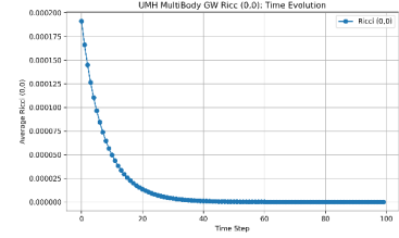
Figure 71: RESULT: Time evolution of the Ricci tensor component R_{00} for the multibody gravitational wave test. The curve shows the expected decay and stabilization after soliton interaction, consistent with UMH theoretical predictions.
