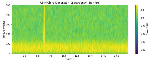
Figure 59: RESULT: UMH Chirp Generator: Spectrogram at Hanford site. Power spectral density shows time–frequency evolution of the simulated chirp signal, with a sharp transient around t \approx 6 s and broadband structure consistent with the modeled UMH waveform.
