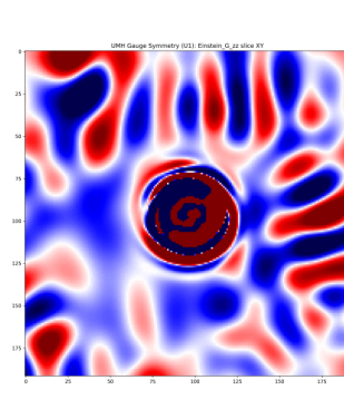
RESULT: U(1) gauge Einstein G_{zz} Slice xy.
