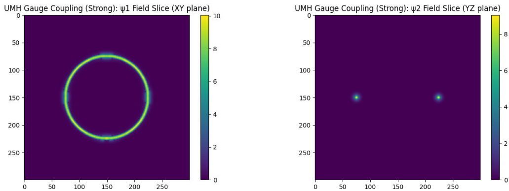
Figure 128: RESULT: Strong SU(3) Field Slices. Orthogonal phase components \psi_1 and \psi_2 demonstrate rotational confinement across distinct planes, mimicking color charge confinement.
