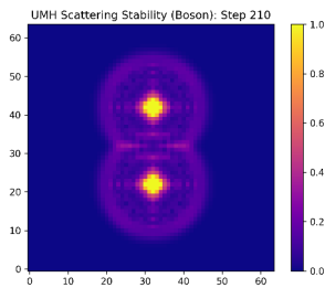
RESULT: Step 210: Separated solitons re-emerge with restored amplitudes and matching phase fronts.
