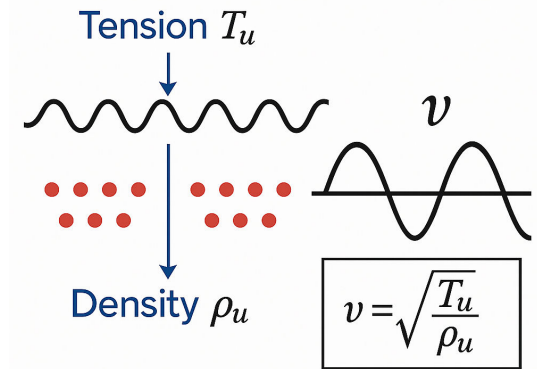
Figure 4: Dimensional derivation of wave speed in the ultronic medium. The relation v = \sqrt{\frac{T_u}{\rho_u}} forms the mechanical foundation from which light speed, gravitational coupling, and Planck's constant are derived.
