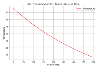
Figure 151: RESULT: Temperature decay curve indicating internal thermalization.
