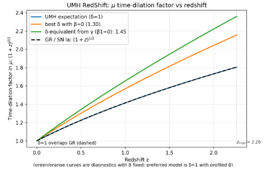
Figure 155: RESULT: Time-dilation factor in the Hubble prediction. In the UMH expression \mu(z) = 5 \log_{10}(d(1+z)^{(1+\delta)/2}/\sqrt{T(z)}) + 25 , the (1 + z)^{(1+\delta)/2} term encodes time dilation. With \delta = 1 , the curve tracks the SN Ia reference; attenuation T(z) handles the remaining flux evolution.
