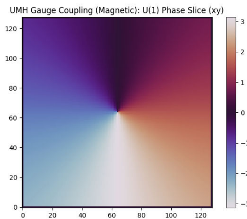
Figure 121: RESULT: Magnetic Phase Structure (XY Slice). The central loop induces a smooth circulating phase profile. This field corresponds to the magnetic vector potential under UMH mechanics.
