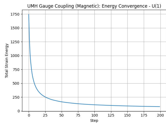
Figure 120: RESULT: Magnetic U(1) Energy Convergence. Total strain energy decreases with relaxation steps, indicating stable coupling dynamics and convergence of the simulated phase configuration.
