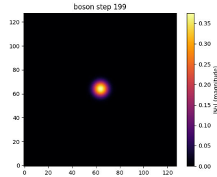
Figure 92: RESULT: Bosonic central peak from condensate collapse.
