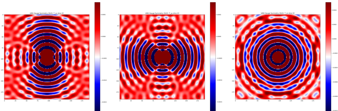
Figure 108: RESULT: Stress-energy components T_{xx} , T_{yy} , and T_{zz} for SU(2) test. Localized solitonic stresses confirm gauge-mediated curvature.
