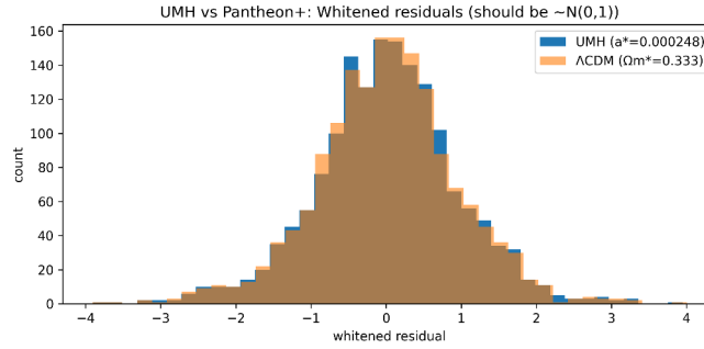
Figure 82: RESULT: Whitened residual distributions for UMH and \Lambda CDM (full STAT+SYS covariance). Both are close to \mathcal{N}(0, 1) ; UMH has |r| smaller than \Lambda CDM for 47.7% of SNe.
