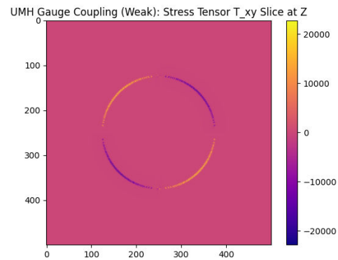
Figure 126: RESULT: Weak-coupling shear component T_{xy} . Off-diagonal shear pattern tracing orthogonal phase constraints.
