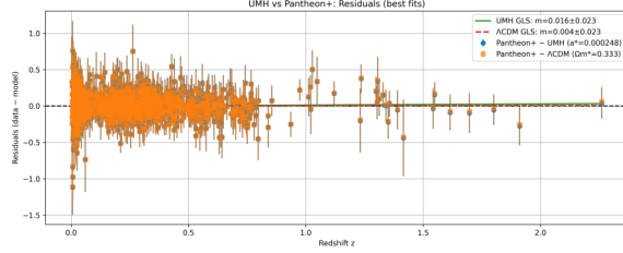
Figure 80: RESULT: Residuals (data–model) vs. z for UMH and \Lambda CDM. GLS trend lines are consistent with zero (UMH: 0.016 \pm 0.023 ; \Lambda CDM: 0.004 \pm 0.023 ).
