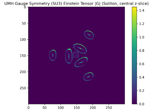
Figure 138: RESULT: UMH Gauge Symmetry (SU3): Einstein tensor magnitude field near soliton. Spatial agreement with known T_{\mu\nu} sources confirms correct curvature generation and conservation.
