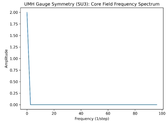
Figure 101: RESULT: SU(3) core — frequency domain. Quantized mode structure from topological phase-lock.
