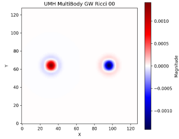
Figure 69: RESULT: Ricci Tensor R_{00} component slice at final step. Peak curvature aligns with injected soliton centers, confirming localized gravitational interaction.
