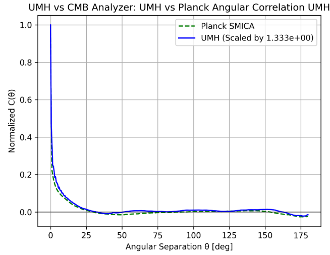
Figure 76: RESULT: Angular correlation function C(\theta) of the UMH-projected CMB anisotropies. The alignment of the angular turnover at \sim 155^\circ with Planck observations confirms that UMH's causal wave interactions naturally reproduce the observed CMB acoustic horizon without inflationary assumptions or parameter fitting.
