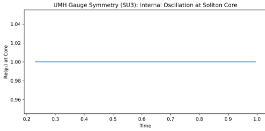
Figure 100: RESULT: SU(3) core — field oscillation. Field oscillation at the soliton core.
