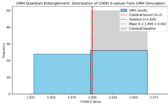
Figure 130: RESULT: Histogram of CHSH S across N = 50 independent-settings UMH runs. Vertical markers indicate the classical bound ( S = 2 ) and the Tsirelson bound ( 2\sqrt{2} ). The sample mean is 1.9995 \pm 0.0028 (SEM), clustering tightly around 2.
