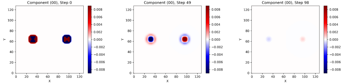
RESULT: UMH MultiBody GW Einstein Frame 000
