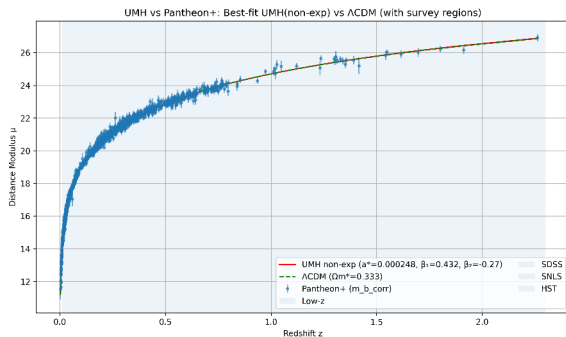
Figure 78: RESULT: Hubble diagram: best-fit UMH (red; minimal calibration—only M profiled) and flat \Lambda CDM (green, dashed; free \Omega_m , profiled M ) over Pantheon+ ( N = 1624 ). Curves are visually indistinguishable; survey regions annotated.
