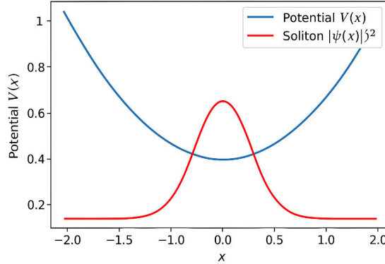
Figure 5: Nonlinear potential V(x) (blue) and soliton energy density |\psi(x)|^2 (red). The soliton remains confined within the potential minimum, stabilized by nonlinear mechanical restoring forces in the ultronic medium.
