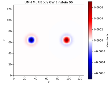
Figure 70: RESULT: Einstein Tensor G_{00} response field showing strain superposition from dual soliton configuration. Symmetry reflects conservation under UMH interaction laws.
