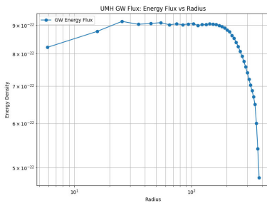
Figure 145: RESULT: UMH GW Flux: Energy Flux vs Radius. Note the near-field plateau and the sharp decrease near the boundary.
