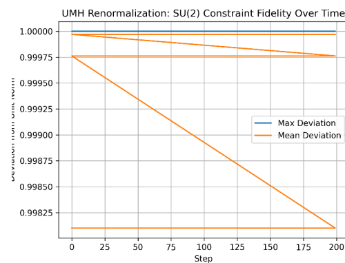
Figure 149: RESULT: Deviation from SU(2) norm over time. Higher resolution grids exhibit reduced phase error.
