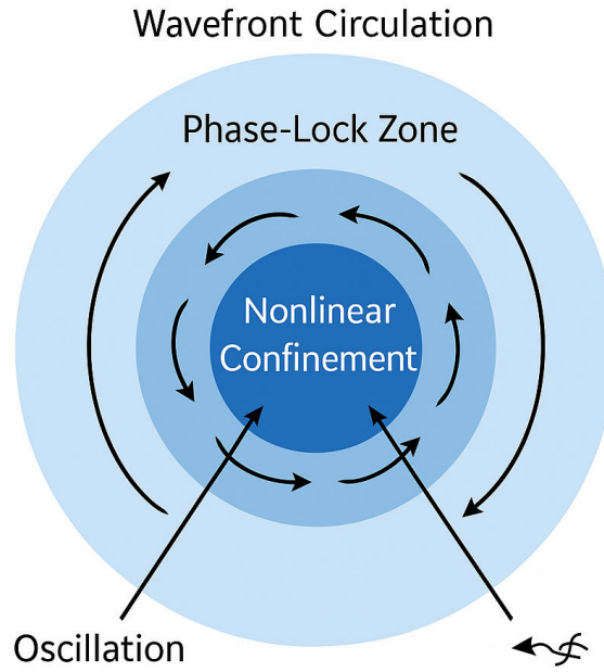
Figure 153: Soliton Wave Structure Anatomy. Schematic of the internal structure of a soliton in the ultronic medium. Phase-locked circulating wavefronts maintain stability, with nonlinear strain confinement preventing dispersion. This structure underlies the emergence of mass, spin, and charge from mechanical wave behavior in the UMH framework.
