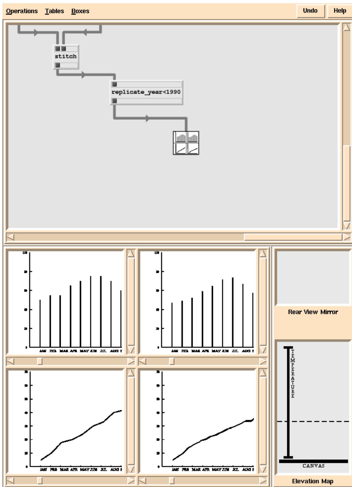
Figure 11: A replicated viewer.
