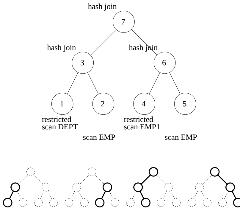
Figure 8. A sample bushy query plan tree and its fragments.
