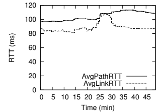
Figure 13: RTTs (with smoothing).
