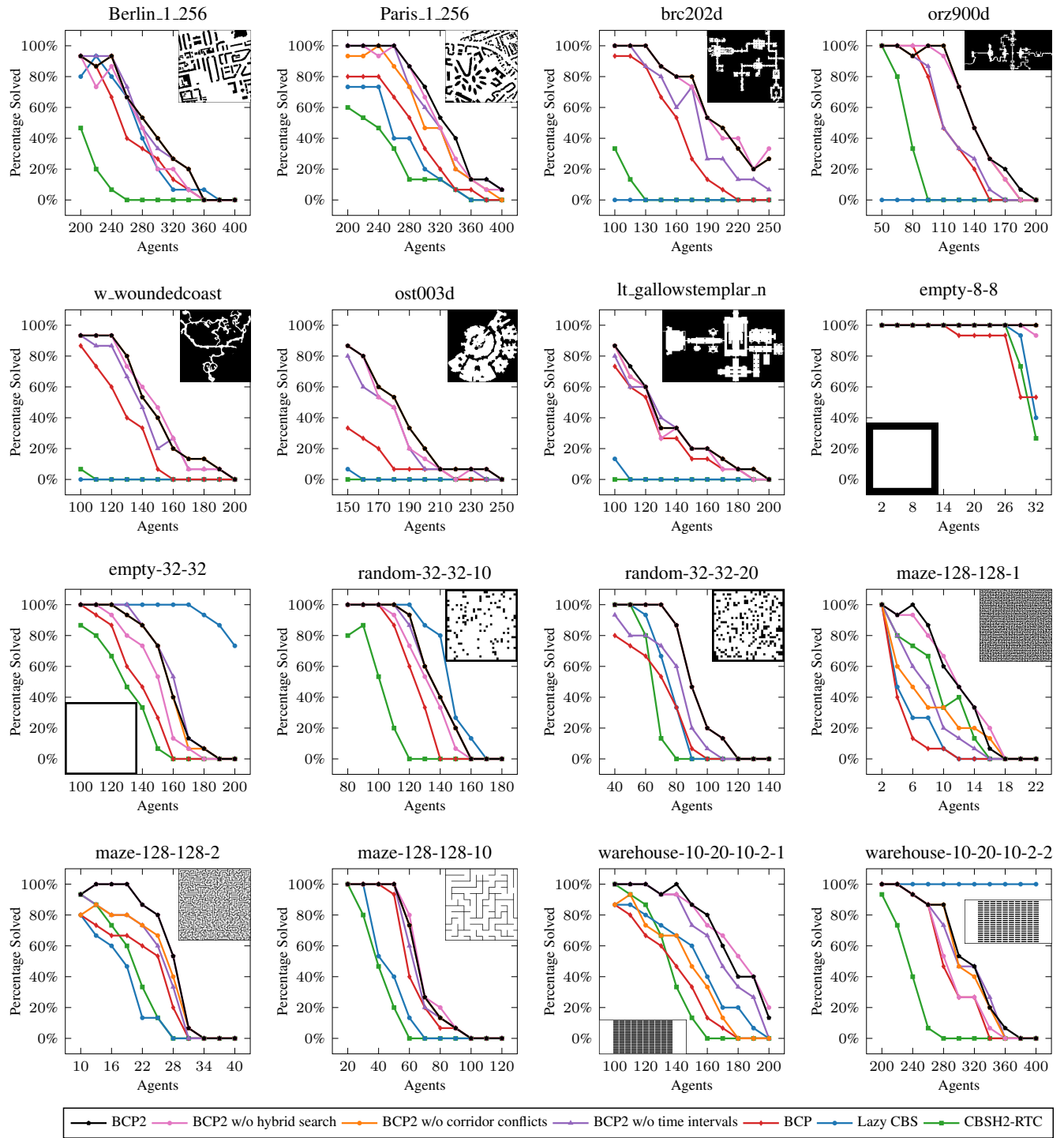
Figure 3: Success rate of the algorithms by map. Higher is better.
