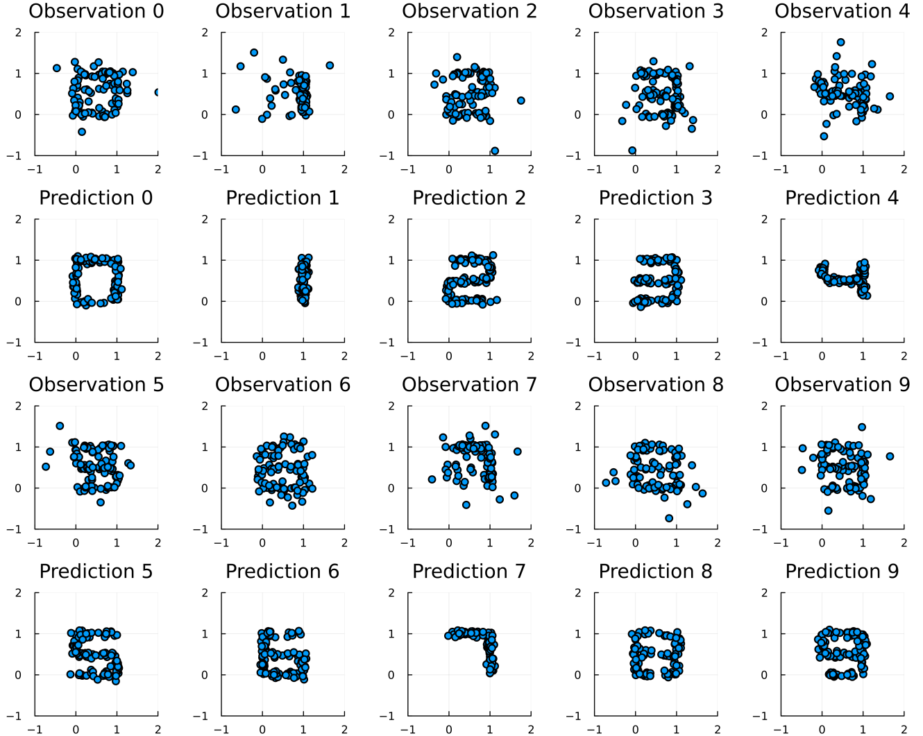
Figure 4: Model Predictions of Digits. Given noisy observations of digits, we infer the base digit and produce a denoised version of the observations. We represent each digit as a collection of 2D Gaussians, each parameterizing a line on the digit.
