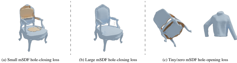
Figure 17: Extreme cases with inappropriate mSDF regularization scales.
