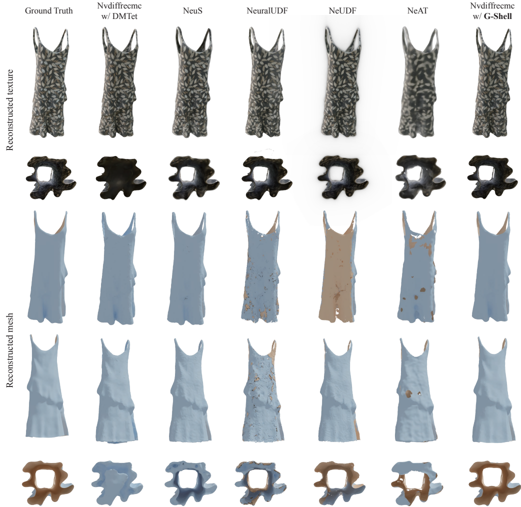
Figure 12: Comparison between reconstruction w/ G-SHELL and baseline methods on multiview reconstruction on instance 117 in DeepFashion3D dataset.
