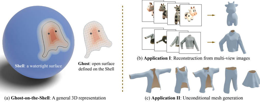
Figure 1: Left: Illustration of mesh extraction with G-SHELL through a manifold signed distance on a surface; Right: Applications of G-SHELL , multiview mesh reconstruction (top) and mesh generation (bottom).
