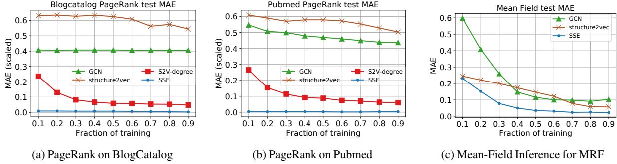
Figure 3. Algorithm learning for PageRank and Mean Field Inference. Error is measured using Mean Absolute Error (MAE).
