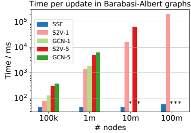
(a) Wall-clock time per round of update. The (*) in the figure denotes the out-of-memory error.
