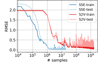
(c) Convergence on BA graphs with # nodes=1,000,000 and m=4.
