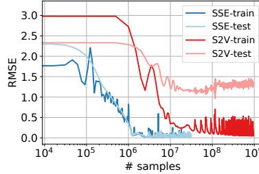
(b) Convergence on BA graphs with # nodes=1,000,000 and m=1.
