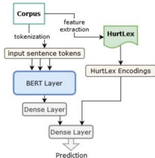
Figure 1: HurtBERT-Enc, our model using HurtLex Encodings
