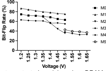
Fig. 10. Bit-flip rate on tested modules when DRAM supply voltage is tuned.
