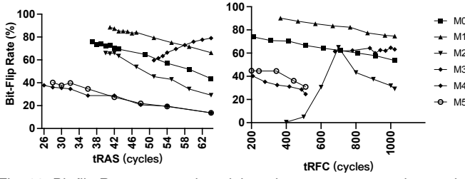
Fig. 12. Bit-flip Rate on tested modules when t_{RAS} or t_{RFC} is tuned.
