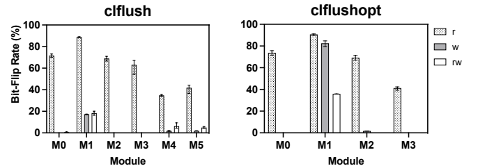
Fig. 5. Bit-flip rate on tested modules when different flush-based hammer methods are applied. The DDR3 modules of M4 and M5 are not illustrated in the right plot as the DDR3-based platform does not support clflushopt instruction.
