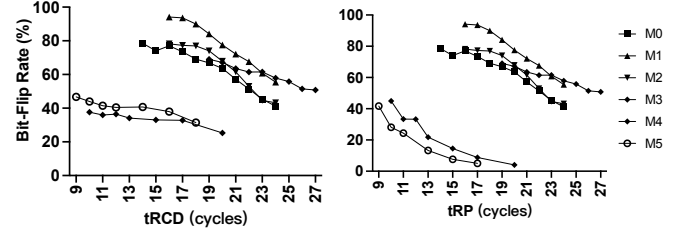
Fig. 11. Bit-flip Rate on tested modules when t_{RCD} or t_{RP} is tuned.
