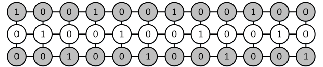
Fig. 3. "Killer" data pattern. The sandwiched victim row looks as '0x492492...' in hexadecimal.
