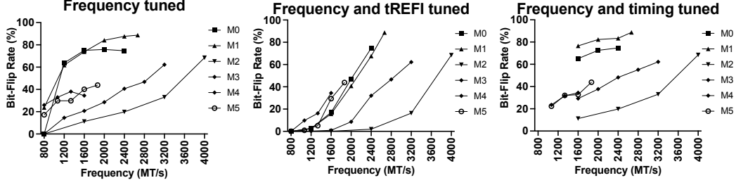
Fig. 9. Bit-flip rate on tested modules when frequency and different timing parameters are tuned. The right plot omits some low frequency cases because the BIOS cannot adjust timings to keep the same memory access latency.
