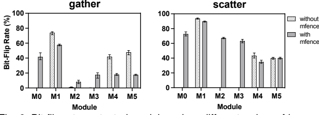
Fig. 6. Bit-flip rate on tested modules when different orders of hammer instruction sequence are applied.
