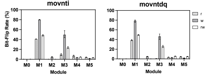
Fig. 4. Bit-flip rate on tested modules when different non-temporal-based hammer methods are applied.
