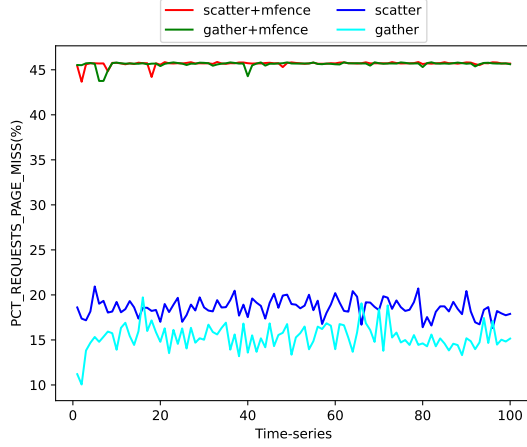
Fig. 8. A comparison of different instruction sequences with regard to the percentage of row buffer conflicts they induced every 50 milliseconds in a given period of 5 seconds.
