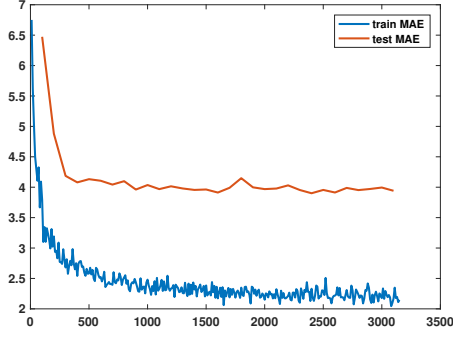
Fig. 3: Training error and testing error of one trial.
