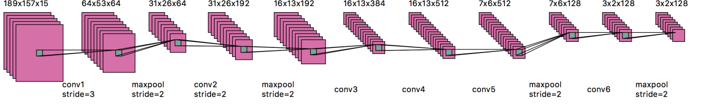
Fig. 1: The first part of our network architecture. Also known as feature extractor. The input slices are represented by the leftmost stacks. After the operations, the information in the slices is represented by a 3 \times 2 \times 128 tensor. Each operation (conv, maxpool) is associated with a stride parameter, which controls how many units the filter shifts at a time. After training, the filter of the convolution will be learned. Note that due to page layout, the number of slices shown in this figure is not accurate and the last 3 fully connected layers are not drawn.
