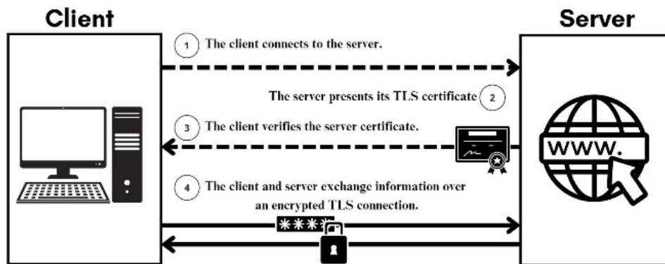
Fig.2. TLS authentication
