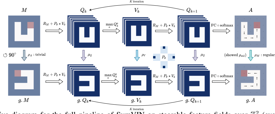
Figure 2: Commutative diagram for the full pipeline of SymVIN on steerable feature fields over \mathbb{Z}^2 (every grid). If rotating the input map M by \pi_M(g) of any g , the output action A = \text{SymVIN}(M) is guaranteed to be transformed by \pi_A(g) , i.e. the entire steerable SymVIN is equivariant under induced representations \pi_M and \pi_A : \text{SymVIN}(\pi_M(g)M) = \pi_A(g)\text{SymVIN}(M) . We use stacked feature fields to emphasize that SymVIN supports direct-sum of representations beyond scalar-valued.
