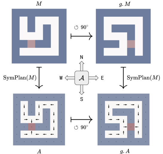
Figure 1: The path planning problem has symmetry, so we study how to exploit its symmetry in (differentiable) planning . Red dots are goal. The optimal actions A = \text{SymPlan}(M) (bottom row) for the maps M (top row) are guaranteed to be equivariant \text{SymPlan}(g.M) = g.\text{SymPlan}(M) under \odot rotations for (2D) path planning. For example, the action in the NW corner of A is the same as the action in the SW corner of g.A , after also rotating the arrow \odot 90^\circ .
