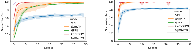
Figure 4: Training curves on (Left) 2D navigation with 10K of 15 \times 15 maps and on (Right) 2DoFs manipulation with 10K of 18 \times 18 maps in configuration space. Faded areas indicate standard error.
