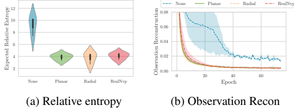
Figure 1: Comparison of priors under normalising flows.
