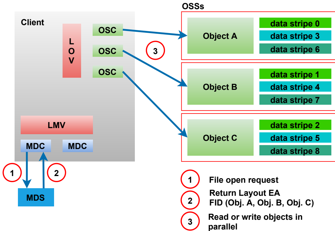
Figure 5. Lustrer I/O operation: Lustrer client requesting file data.
