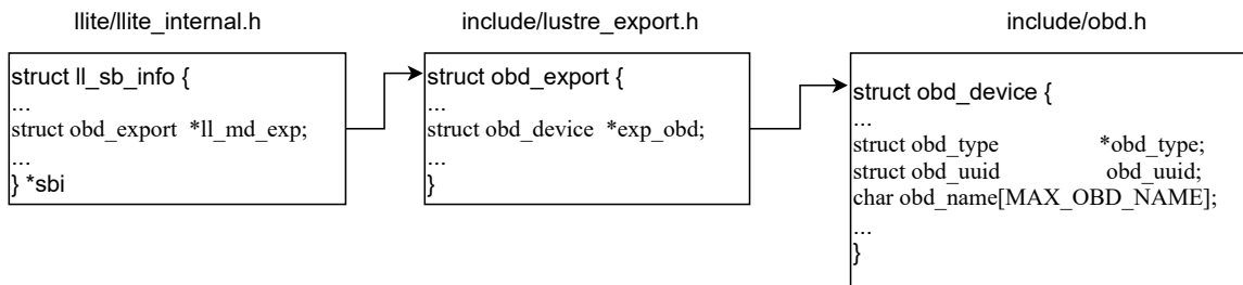
Figure 7. Data structures involved in the communication between mgc and llite subsystems.
