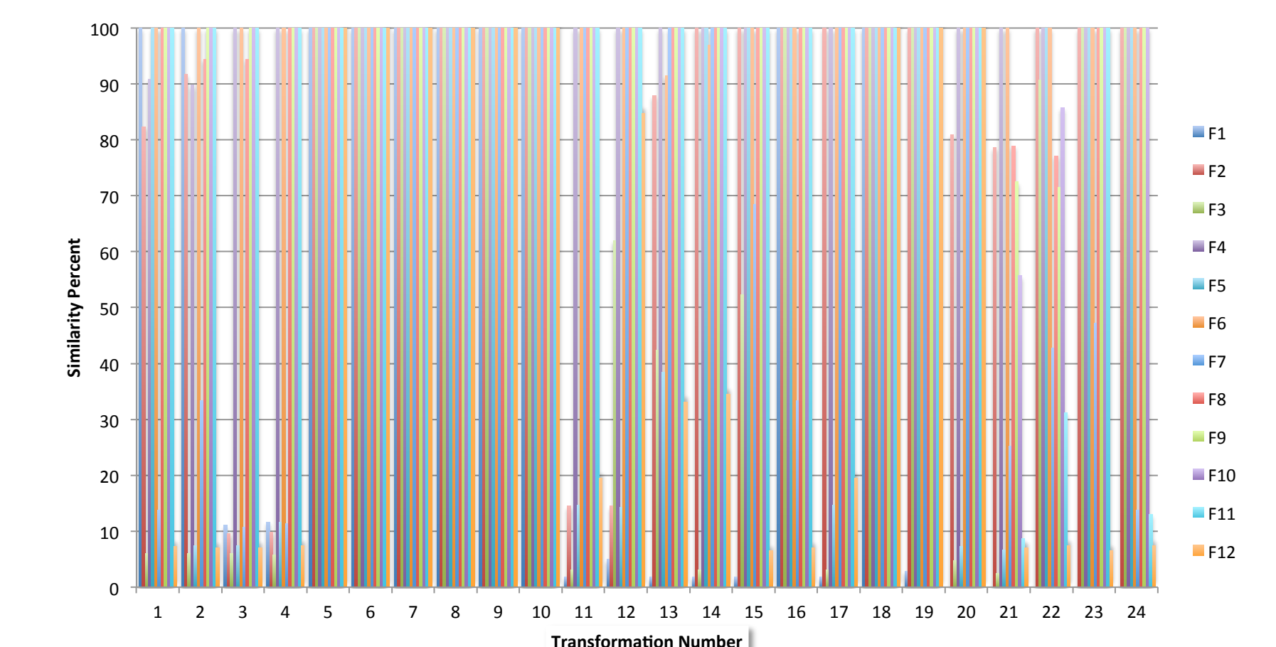
Figure 3: LCS between successive versions of the various functions of the Bzip2 benchmark.
