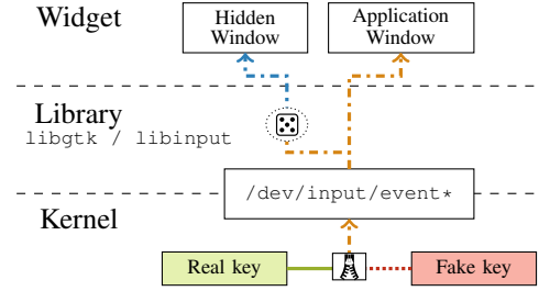
Fig. 5. Multi-layered design of KeyDrown .
