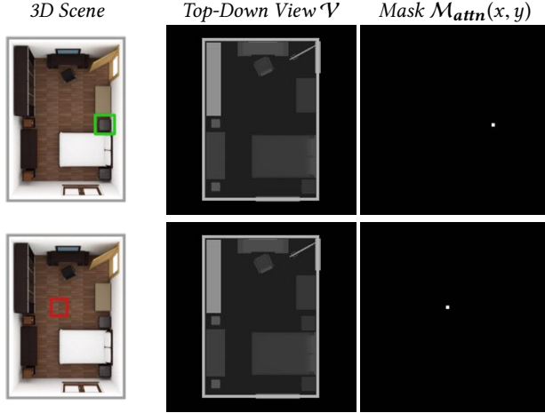
Fig. 5. Illustrating the training examples (x, y, c) used to train CategoryLocation. The colored boxes are centered around the location (x, y) . Top : an example where c = \text{'nightstand'} . The third column shows the attention mask M_{\text{attn}}(x, y) . Bottom : an example where c = \text{'no object'} .
