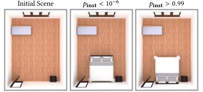
Fig. 8. Using the InstanceOrientation network to predict the validity of inserting model instances at different orientations. Inserting the double bed at the correct orientation with respect to the wall has probability near 1, whereas the opposite orientation is clearly recognized as being incorrect with probability near 0.
