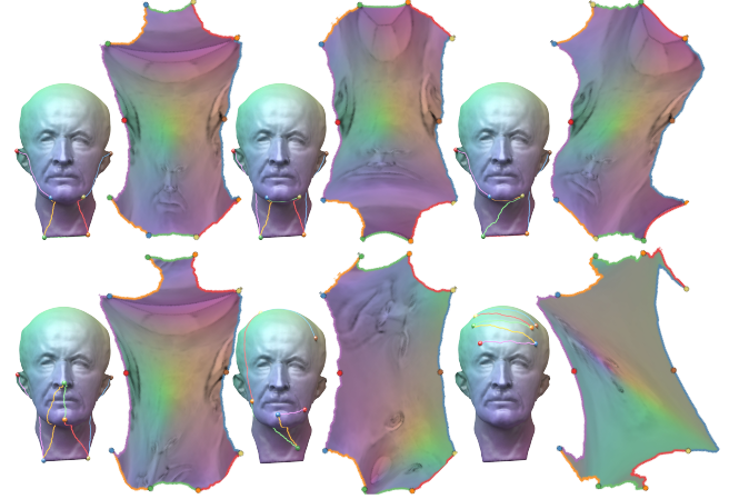
Figure 7: Embeddings into a 6-coned hyperbolic orbifold, each embedding resulting from a different selection of cones.
