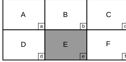
Figure 3: To compute the two-rectangle horizontal feature E - F , we note that the the sum of the pixels in box E can be described using the pixels of the integral image, a + e - b - d , and F is b + f - c - e .
