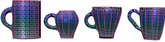
Figure 3: Corresponding feature curves (red) on a set of cups with texture coordinates mapped by the functional map. The left object is the source shape while the other shapes are target meshes.
